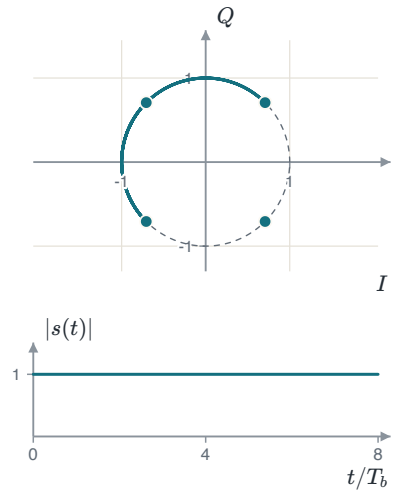
FIGURE 5.31 MSK: the path stays on the circle, and the envelope is constant.
