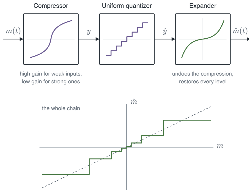
FIGURE 1.46 The quantizer in the middle is uniform. Seen from m to \hat{m} , its steps are fine near zero and coarse near the peak.
