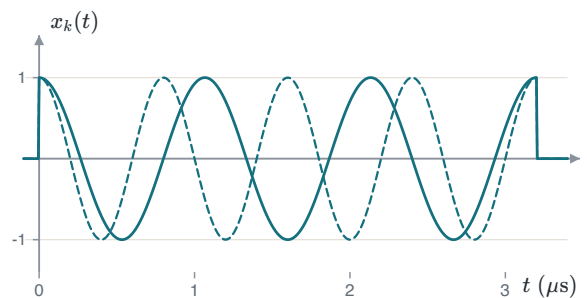
FIGURE 3.9 Wi-Fi spaces its subcarriers \Delta f = 312.5 kHz apart. Over one symbol of T = 1/\Delta f = 3.2 \mu s, \cos(2\pi k \Delta f t) for k = 3 and k = 4 are orthogonal.
