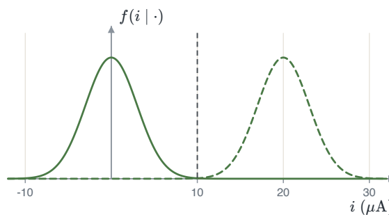
FIGURE 4.23 An optical receiver sees 0 or 20\text{ }\mu\text{A} . The energy term puts the threshold at 10\text{ }\mu\text{A} . With \sigma = 3\text{ }\mu\text{A} , P_e = Q(10/3) = 4.3 \times 10^{-4} .
