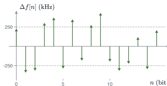
FIGURE 4.25 Bluetooth Low Energy shifts the carrier by about \pm 250 kHz. With equal priors the receiver decides by the sign of each sample.
