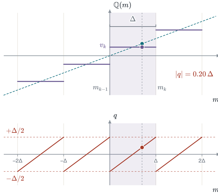
FIGURE 1.31 The error is the gap between the line v = m and the staircase, shown at m = 0.7\Delta . It is largest at a boundary, where it equals \Delta/2 .
