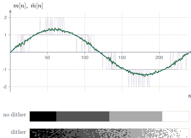
FIGURE 1.40 A slow sinusoid 1.3 steps high through a quantizer with a unit step. The faint traces are the staircase without dither and one output with dither. The green trace averages 64 dithered outputs. The strips are a grey ramp at four levels, without and with dither.
