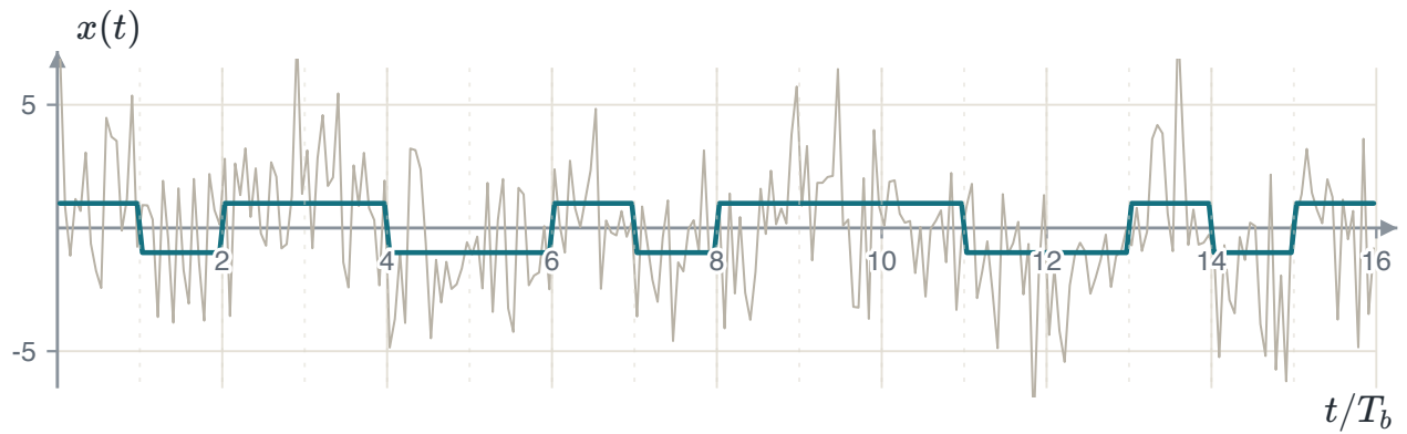
FIGURE B.5 Sixteen bits at E_b/N_0 = 2 dB. The clean square wave is the transmitted s(t) . The hairline around it is x(t) = s(t) + w(t) . This is everything the receiver is given. Nothing about the square wave is visible in the hairline at this noise level, and that is the honest picture. The receiver does not see the signal, it computes with it.
