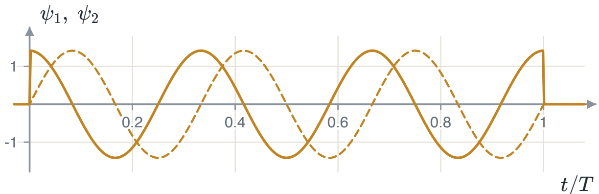
FIGURE 3.8 The two axes with T = 1 and f_c T = 3 : \psi_1 solid and \psi_2 dashed. Each holds whole cycles in [0, T] .
