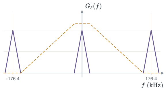
FIGURE 1.21 Oversampling CD audio by four moves the first copy to 176.4 kHz. A gentle filter (dashed) then removes it.
