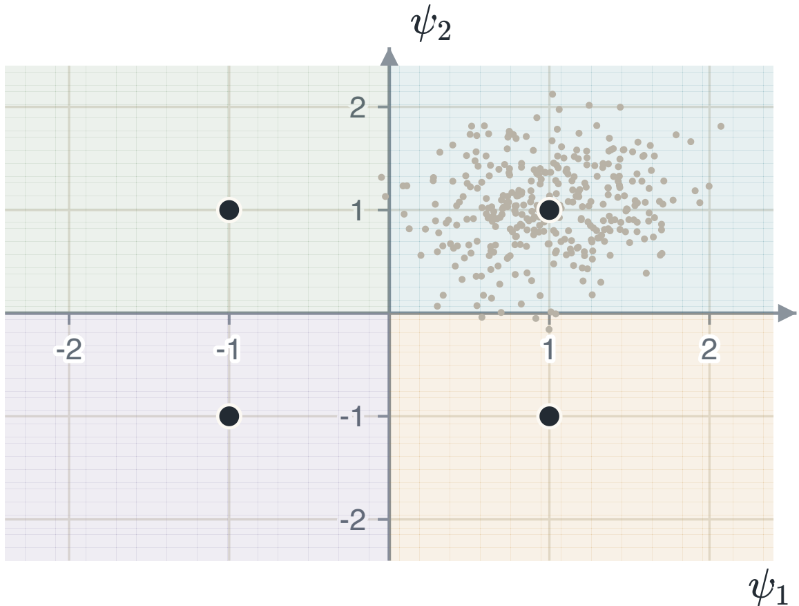
FIGURE 4.4 The constellation, its four regions, and the observations the receiver sees when the top-right point is sent. The exact error probability is the fraction of that cloud outside its own region. The bound adds three separate two-point questions and counts the overlaps twice.
