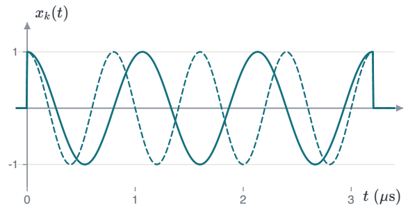
FIGURE 3.9 Wi-Fi spaces its subcarriers \Delta f = 312.5 kHz apart. Over one symbol of T = 1/\Delta f = 3.2 \mu\text{s} , \cos(2\pi k \Delta f t) for k = 3 and k = 4 are orthogonal.
