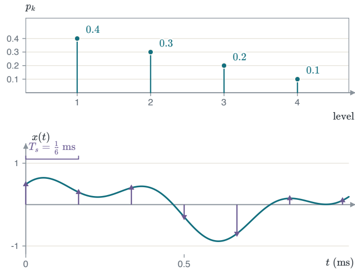
FIGURE 6.5 Top: the four levels of Example 6.1 and their probabilities. Bottom: a source band-limited to 3 kHz, sampled every T_s = \frac{1}{6} ms, which is 6000 samples a second.
