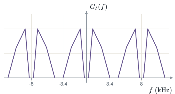
FIGURE 1.9 Telephone speech is filtered to 3.4 kHz and sampled at 8 kHz, which leaves a 1.2 kHz guard band.
