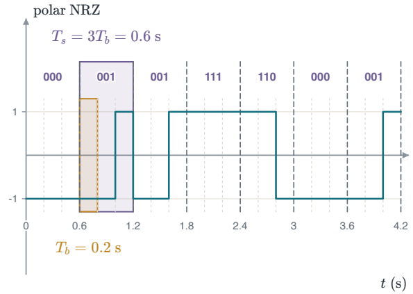
FIGURE 1.54 The seven code words as one polar NRZ stream. The amber box marks one bit, T_b = 0.2\text{ s} . The violet box marks one code word, T_s = 3T_b .
