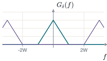
FIGURE 1.1 f_s > 2W : a gap between the replicas.
