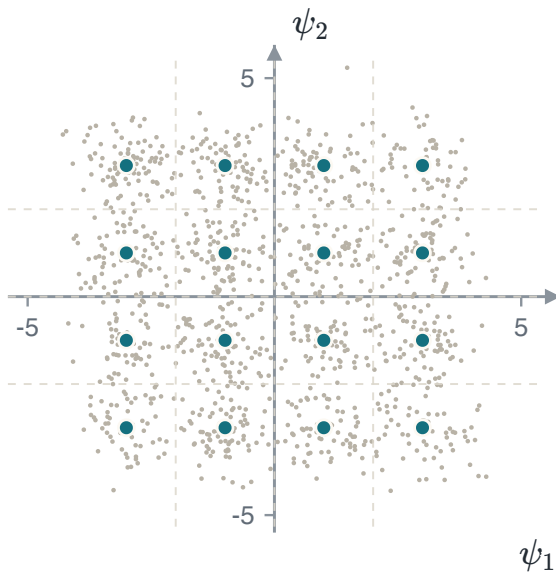
FIGURE 3.1 E_b/N_0 = 6 dB. The clouds touch, so a large fraction of the symbols land across a boundary. The measured symbol error rate here is 0.108: about one symbol in nine is decided wrongly.
