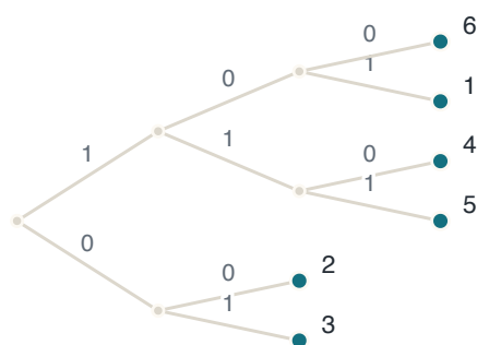
FIGURE 4.2 The code the algorithm builds. Reading a path from the root, left is a 0 and right a 1. The digit at each leaf is the symbol that path spells.
