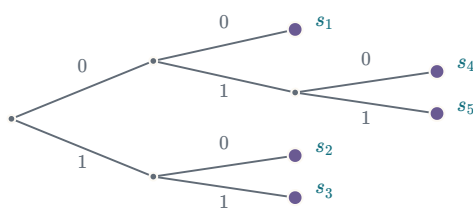
FIGURE 6.5 The Huffman code with ties placed high. Lengths 2, 2, 2, 3, 3 and variance 0.16.
