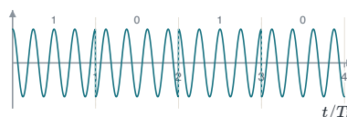
Phase-shift keying: the carrier is always on and its sign flips.
