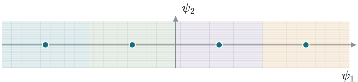
FIGURE 5.7 4-ASK on one axis. The two end regions run off to infinity.
