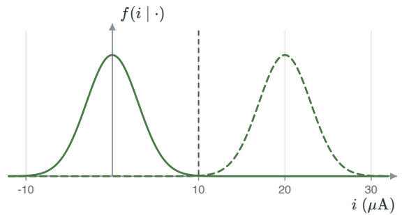
FIGURE 4.23 An optical receiver sees 0 or 20 \mu\text{A} . The energy term puts the threshold at 10 \mu\text{A} . With \sigma = 3 \mu\text{A} , P_e = Q(10/3) = 4.3 \times 10^{-4} .
