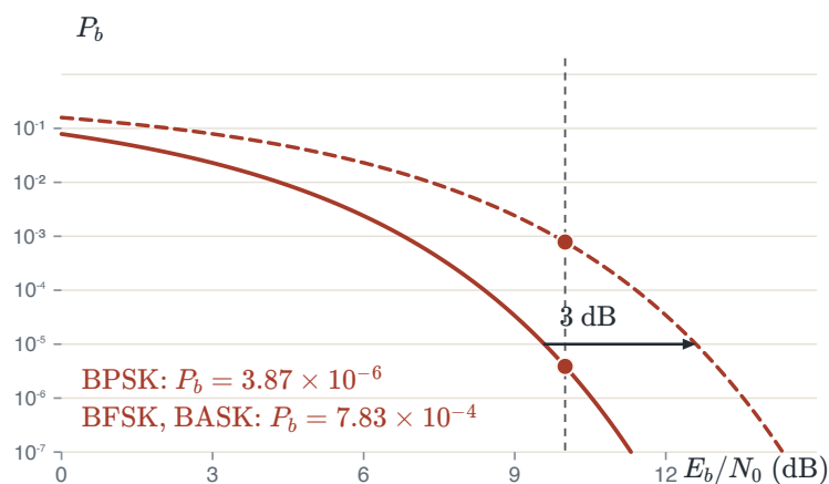
FIGURE 5.6 Bit error of BPSK (solid) and of BFSK and BASK (dashed). At 10^{-5} the dashed curve sits 3 dB to the right. The dots read both curves at E_b/N_0 = 10 dB, the case of Example 5.1.
