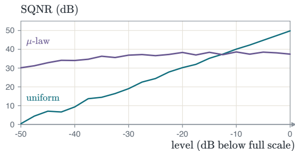
FIGURE 1.49 Two 8-bit quantizers on a sinusoid. The \mu -law SQNR stays nearly flat as the level falls. The uniform one falls a decibel per decibel.
