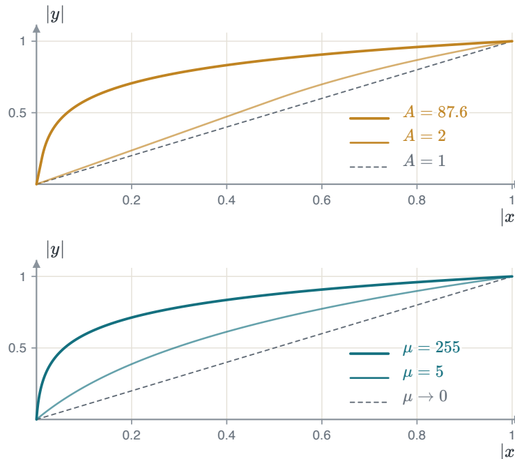
FIGURE 1.48 A-law (top) and \mu -law (bottom) for three parameter values. The dashed line is no companding. The larger the parameter, the more output range goes to small inputs.
