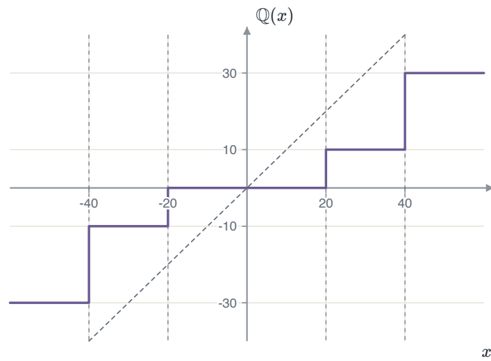
FIGURE 1.39 The five-level quantizer: outputs 0, \pm 10, \pm 30 and boundaries \pm 20, \pm 40 . The dashed line is y = x .
