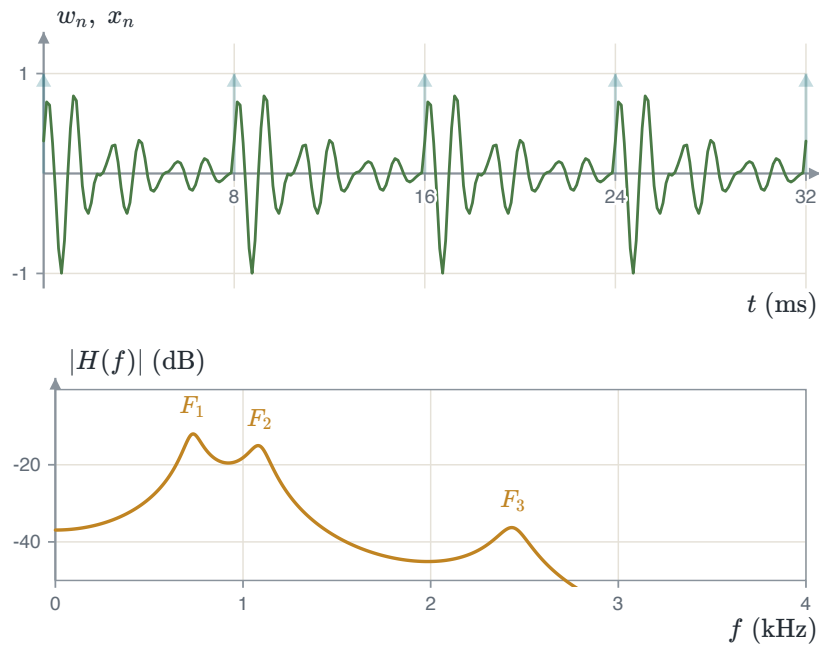
FIGURE 1.66 A pulse train at f_0 = 125 Hz (faint) drives an all-pole filter with three peaks, the formants F_1, F_2, F_3 . The output is a vowel (green). Noise through the same filter is a whisper.
