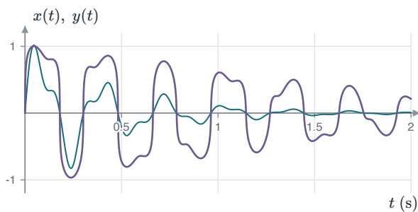
FIGURE 1.51 A decaying burst (cyan) and its \mu -law compressed form (violet). The quiet tail is lifted toward full scale.
