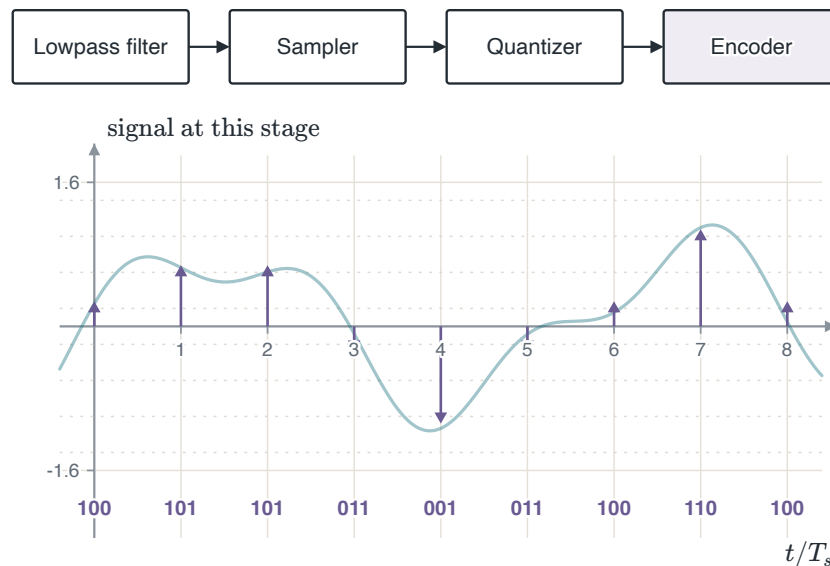
FIGURE 1.70 One message through the four stages. The filter has removed a fast ripple, and the sampler has kept one value every T_s . The quantizer has moved each value to one of eight levels, and the encoder has written three bits for it.
