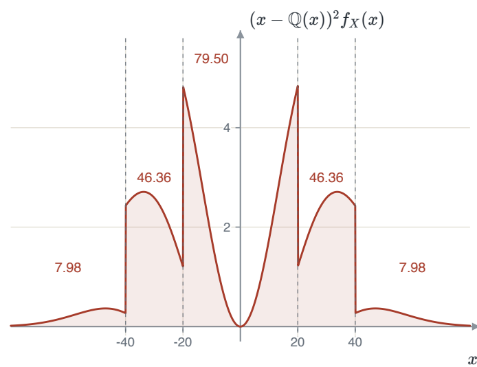
FIGURE 1.40 The error integrand (x - Q(x))^2 f_X(x) , region by region. The five areas add to the noise power P_Q = 188.17 .
