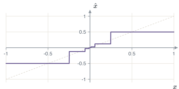
FIGURE 1.52 A 3-bit \mu -law quantizer drawn against its input: narrow steps near zero, wide steps near the peak.
