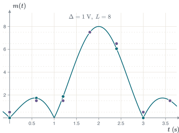
FIGURE 1.54 The message (cyan), its samples every 0.6 s, and the selected levels (violet). Each error is under half a step.
