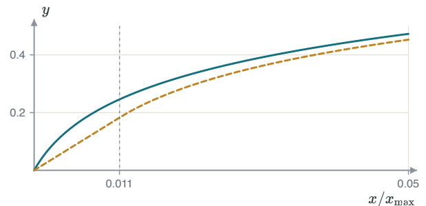
FIGURE 1.50 Near zero the laws differ: A-law is a straight line up to 1/A = 0.0114 , and \mu -law is curved all the way.
