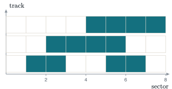
FIGURE 1.63 A shaft encoder prints a Gray code on three tracks. At each sector edge only one track changes.
