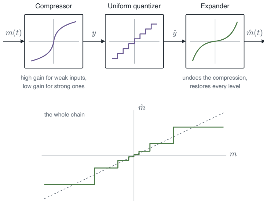
FIGURE 1.47 The quantizer in the middle is uniform. Seen from m to \hat{m} , its steps are fine near zero and coarse near the peak.
