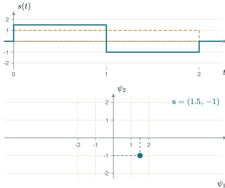
FIGURE 3.3 The waveform s_1\psi_1(t) + s_2\psi_2(t) and the point (s_1, s_2) , drawn for s_1 = 1.5 and s_2 = -1 . The dashed pulses are \psi_1 and \psi_2 .
