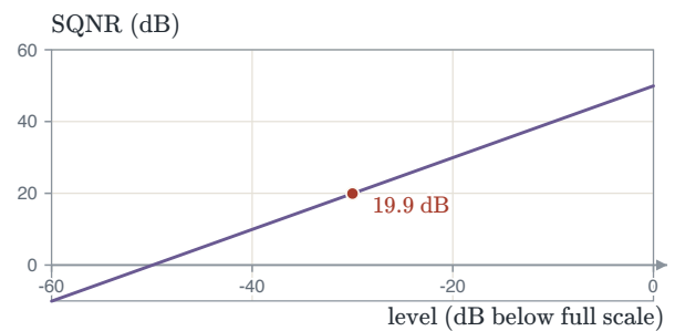
FIGURE 1.43 By \alpha + 6.02R , uniform 8-bit PCM gives 49.9 dB at full scale but only 19.9 dB for a signal 30 dB below it.
