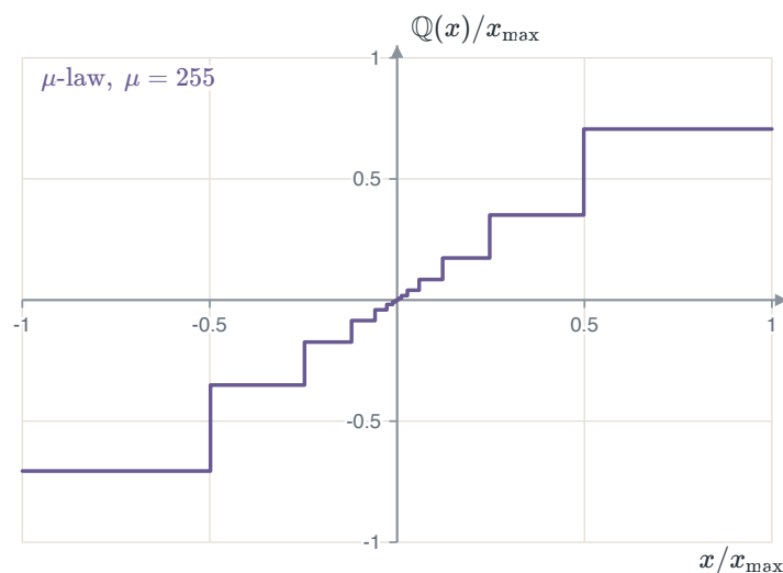
FIGURE 1.46 A sixteen-level \mu -law quantizer. Its steps are fine near zero, where speech amplitudes crowd, and coarse near the peak.
