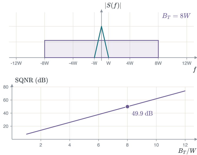
FIGURE 1.56 Top: the message band W (cyan) and the least band of 8-bit PCM sampled at 2W (violet). Bottom: the SQNR of a full-scale sinusoid against that bandwidth.
