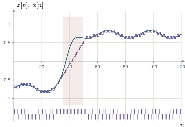
FIGURE 1.59 A signal with one steep rise, and the staircase with \Delta = 0.06 that follows it one step a sample. Red shades slope overload. The ticks under the plot are the bits.
