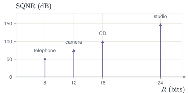
FIGURE 1.45 A full-scale sinusoid at common word lengths: 49.9, 74.0, 98.1 and 146.3 dB.
