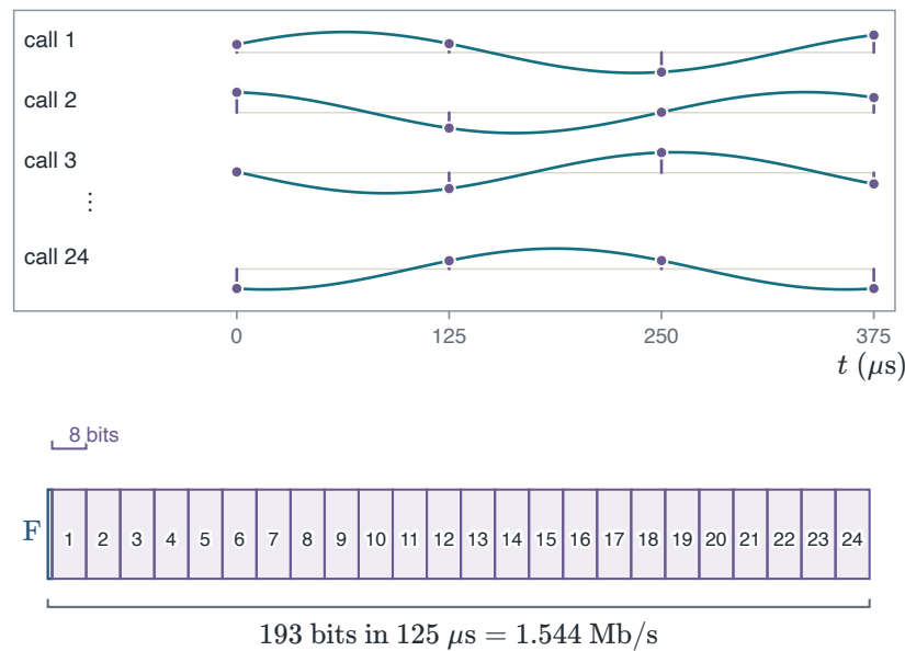
FIGURE 1.67 Every call is sampled every 125 \mu\text{s} . Its 8-bit word takes one slot of the frame, after a framing bit F.
