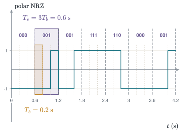
FIGURE 1.55 The seven code words as one polar NRZ stream. The amber box marks one bit, T_b = 0.2 \text{ s} . The violet box marks one code word, T_s = 3T_b .
