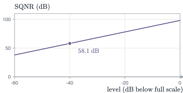
FIGURE 1.42 CD audio uses 16 bits: 98.1 dB at full scale, and 58.1 dB for a passage 40 dB quieter.
