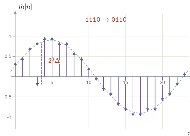
FIGURE 1.57 A 4-bit PCM stream with \Delta = 0.125 . Bit b = 3 of the code word 1110 is received wrong, and the sample moves by 2^3 \Delta .
