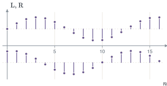
FIGURE 1.60 CD audio: two channels of 16 bits at 44.1 kHz give 2(16)(44\,100) = 1.4112 Mb/s.
