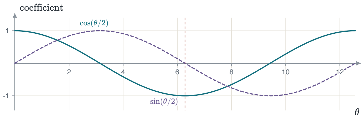
FIGURE 1.7 The two coefficients over two full turns. At \theta = 2\pi the cosine is -1 and the sine is 0, so the operator is -I : the matrix takes twice as long to come home as the state it acts on. The leftover sign is a global phase and no experiment sees it, which is why the two are consistent.
