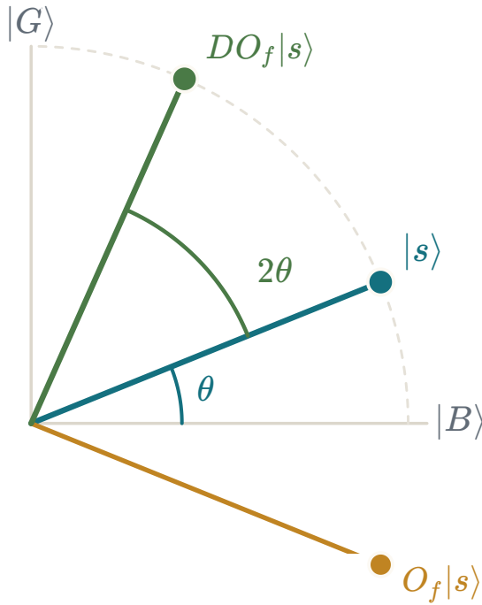
FIGURE 5.6 One iteration, drawn isotropically so the angles are the real ones. The oracle takes the vector below the horizontal; the diffusion takes it back above, but past where it started. The net turn is 2\theta .
