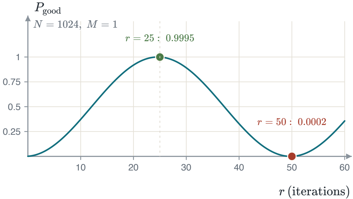
FIGURE 5.7 The success probability against the iteration count, for a thousand candidates with one marked. It rises to almost one at twenty-five iterations and falls back to almost nothing at fifty. The curve is a sine squared and it keeps going.
