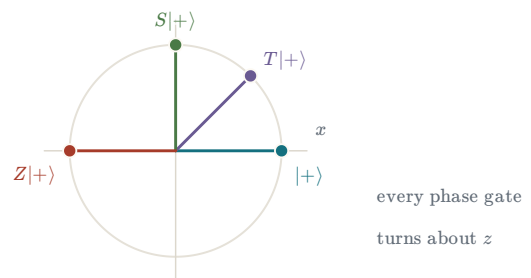
FIGURE 4.7 The equator seen from above, with |+\rangle carried round by T , by S and by Z . Each is the same gate with a different angle.
