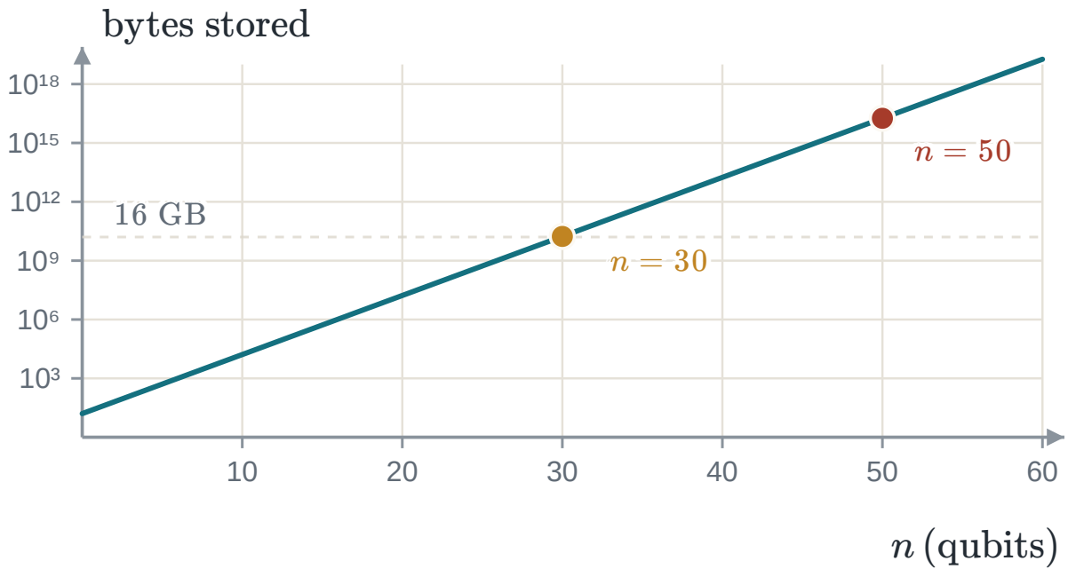
FIGURE 5.3 What one state vector costs, against the number of qubits. The vertical axis is logarithmic, so the exponential is a straight line and no amount of extra hardware bends it.
