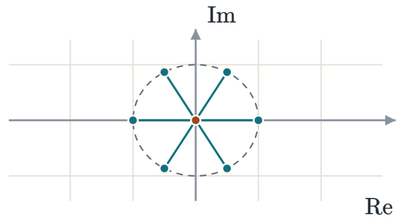
FIGURE 1.53 N = 6, k = 1 : the six terms e^{j\pi n/3} are spread evenly over the circle, and the sum is 0.
