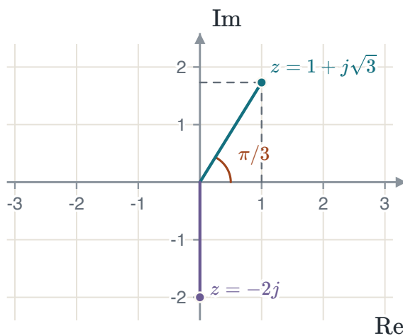
FIGURE 1.34 z = 2e^{j\pi/3} = 1 + j\sqrt{3} lies at distance r = 2 and angle \pi/3 . z = -2j = 2e^{-j\pi/2} lies on the negative imaginary axis.
