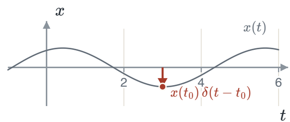
FIGURE 1.33 Sampling: the impulse at t_0 is scaled by the value of x there. Integrating returns that number.
