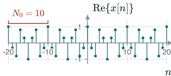
FIGURE 1.46 \text{Re}\{e^{j3\pi n/5}\} repeats every 10 samples.
