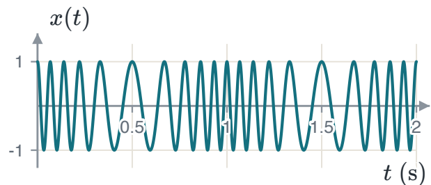
FIGURE 1.69 FM: x(t) = \cos(2\pi f_c t + \beta \sin(2\pi f_m t)) . Drawn with f_c = 10 Hz, f_m = 1 Hz, \beta = 5 .
