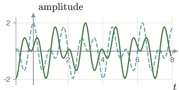
FIGURE 4.7 x(t) = \cos 4t + \cos 7t (dashed) and the delayed output (solid).
