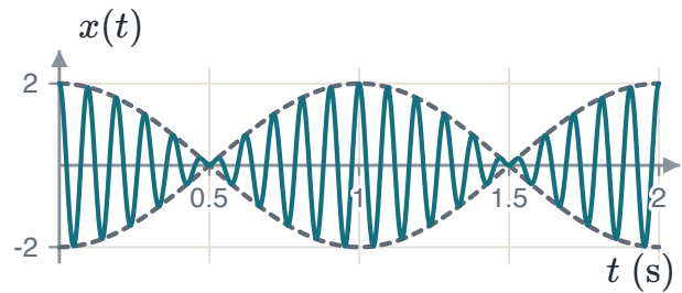
FIGURE 1.67 Beats: \cos(2\pi f_1 t) + \cos(2\pi f_2 t) , drawn with f_1 = 10 Hz, f_2 = 11 Hz. The dashed envelope is \pm 2 \cos(\pi(f_1 - f_2)t) .
