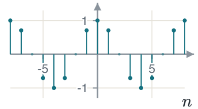
FIGURE 1.45 \omega_0 = 7\pi/4 = 2\pi - \pi/4 : the same samples as \pi/4 .
