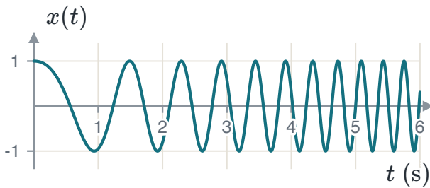
FIGURE 1.66 Chirp: x(t) = \cos(2\pi(f_0t + \frac{k}{2}t^2)) . Its frequency f_0 + kt rises with time. Drawn with f_0 = 0.3 Hz, k = 0.5 Hz/s.
