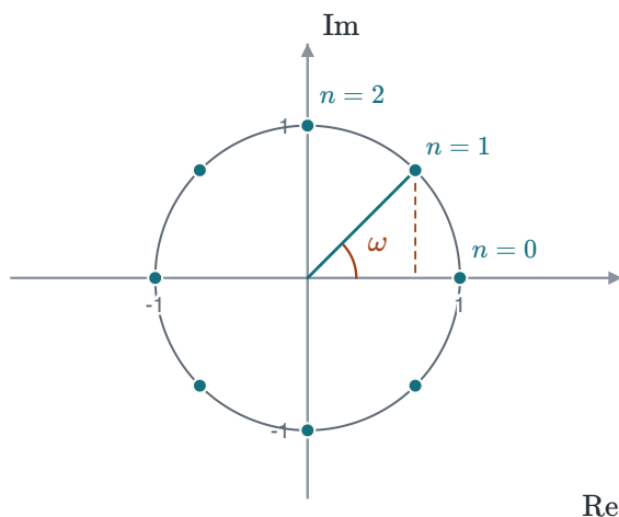
FIGURE 6.7 The points e^{j\omega n} for \omega = \pi/4 : each step turns by \omega , and after eight steps the point is back at 1. The dashed drop gives the real part at n = 1 .
