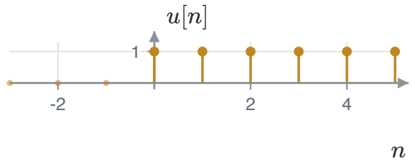
FIGURE 1.30 The unit step u[n] : 1 for n \geq 0 , including u[0] = 1 .
