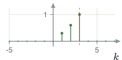
FIGURE 3.6 Shift: h[3-k] , with h[0] at k=3
