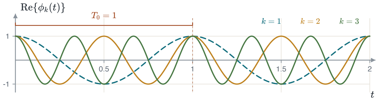
FIGURE 1.49 The harmonics k = 1 (dashed), k = 2 and k = 3 with T_0 = 1 . The k -th makes k full cycles in T_0 , so all of them start together again at t = T_0 .
