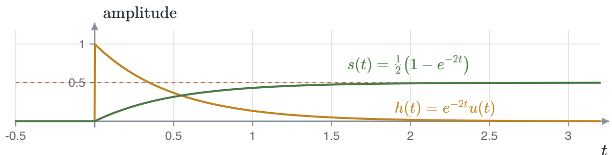
FIGURE 3.26 The impulse response and the step response of y' + 2y = x at rest. The step response settles at \frac{1}{2} , the dashed line.
