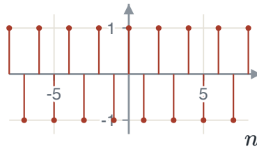
FIGURE 1.44 \omega_0 = \pi : (-1)^n , the fastest.
