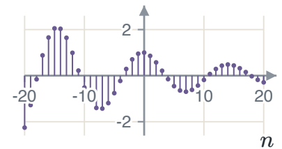
FIGURE 1.42 0.95^n \cos(0.14\pi n) : |\alpha| = 0.95 decays.
