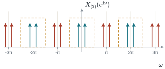
FIGURE 7.63 x_b[n] = \cos(\pi n/4) with one zero inserted after every sample, N = 2 : the wanted lines at \pm\pi/8 , cyan, and the images at \pm7\pi/8 , red, in every period. The low-pass, dashed, keeps |\omega| < \pi/2 .
