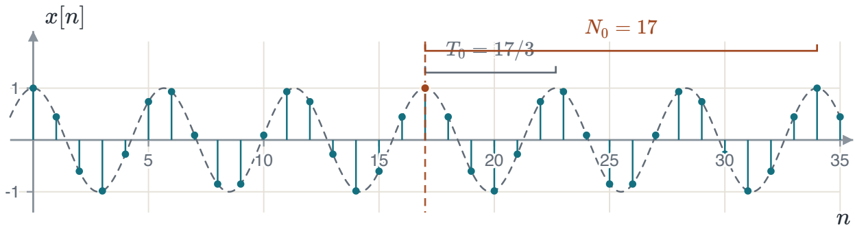
FIGURE 1.48 The dashed curve \cos(6\pi t/17) repeats every 17/3 , but no sample falls at the end of its first or second cycle. After three cycles, at n = 17 , a sample falls on the start of a cycle again. The brackets mark one cycle of the curve and one period of the sequence, both from n = 17 .
