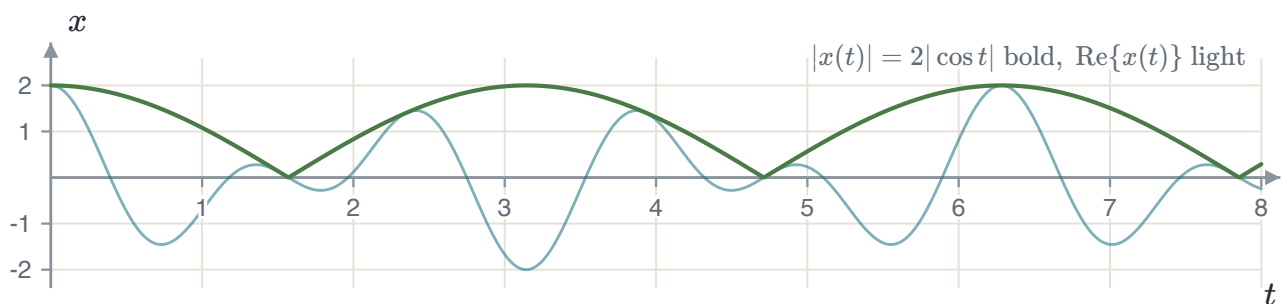
FIGURE 1.39 x(t) = e^{j3t} + e^{j5t} . The magnitude 2|\cos t| repeats every \pi . The real part 2 \cos t \cos 4t oscillates inside it.
