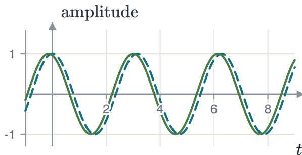
FIGURE 4.6 \cos 2t (dashed) and \cos(2(t-3)) (solid).
