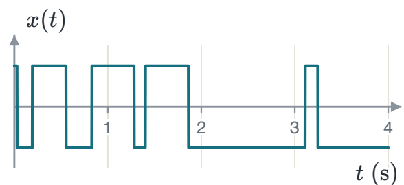
FIGURE 1.73 Random telegraph: x(t) is +1 or -1 and flips sign at random times. Only the times of the flips are random.
