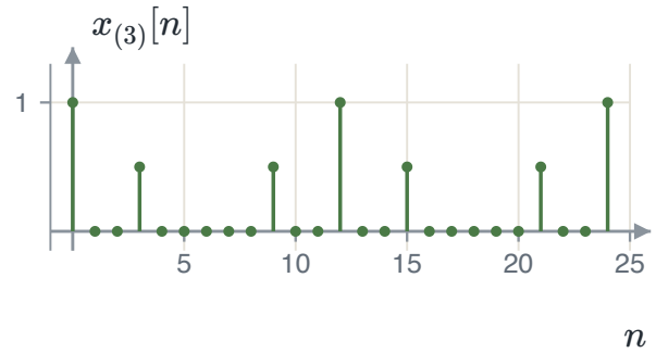
FIGURE 4.52 x_{(3)}[n] : two zeros after each sample, period 12.
