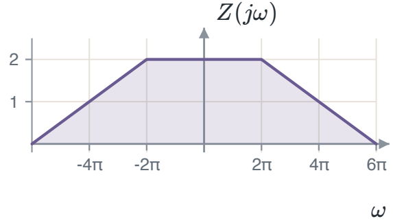
FIGURE 5.31 Example 5.24: the trapezoid, flat on |\omega| \leq 2\pi and zero beyond 6\pi .
