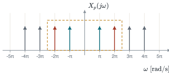
FIGURE 7.37 The lines of Example 7.9 after sampling at \omega_s = 5\pi rad/s, with the filter |\omega| < 2.5\pi dashed. The line at \pi is kept, cyan, the copy line at 2\pi is kept, red, and the grey lines are removed.
