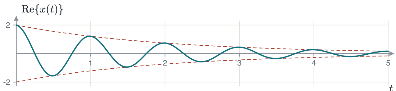
FIGURE 1.38 A damped sinusoid, \text{Re}\{2e^{-0.5t}e^{j2\pi t}\} , with A = 2 , r = -0.5 and \omega_0 = 2\pi rad/s. The envelope \pm 2e^{-0.5t} is dashed.
