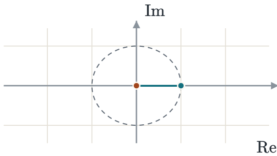
FIGURE 1.52 N = 6, k = 0 : all six terms sit at 1, and the sum is 6.
