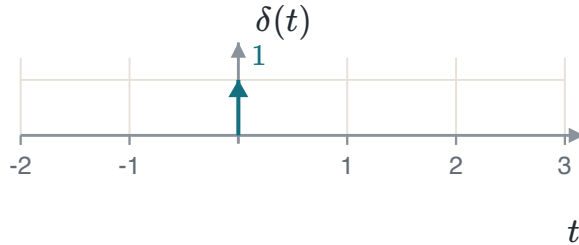
FIGURE 1.32 The arrow height shows the area , never a value of a function.
