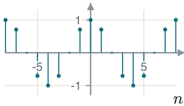
FIGURE 1.43 \omega_0 = \pi/4 : slow.
