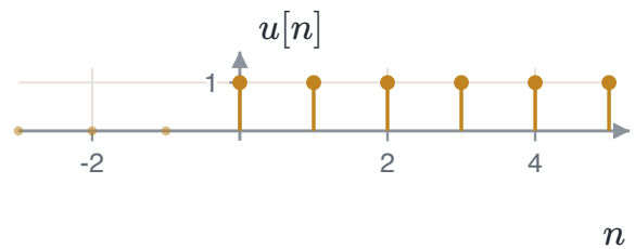
FIGURE 1.31 The unit step u[n] : 1 for n \geq 0 , including u[0] = 1 .
