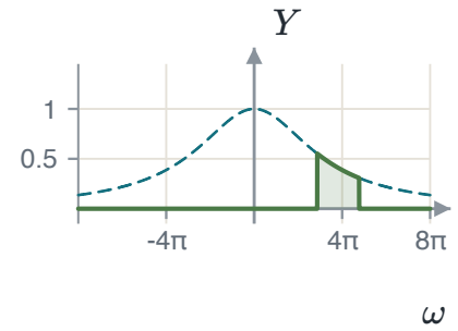
FIGURE 5.29 Shifted back: Y(j\omega) on 9 < \omega < 15 .
