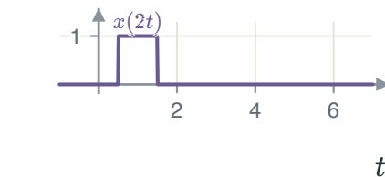
FIGURE 1.14 Compressed: support [0.5, 1.5] .
