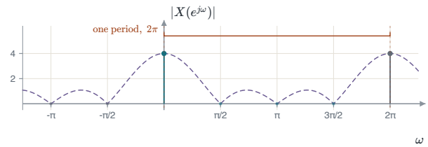
FIGURE 6.10 N = 4 : the stems read 4, 0, 0, 0. Three of them land on zeros of the curve.
