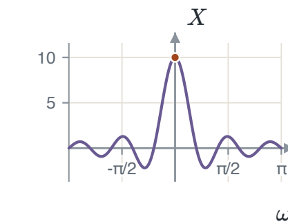
FIGURE 5.10 T_1 = 5 : peak 10.
