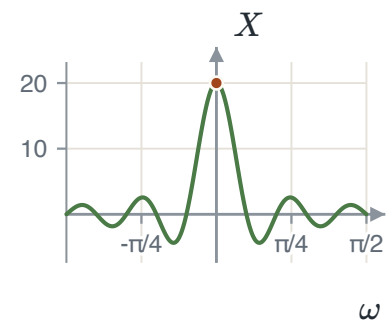
FIGURE 5.11 T_1 = 10 : peak 20.
