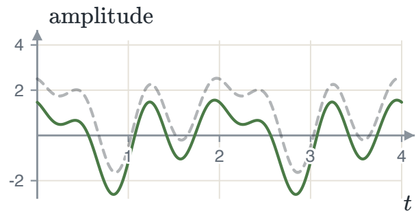
FIGURE 4.69 x(t) (dashed) and y(t) (solid): the harmonics pass almost unchanged and the average drops to 0.
