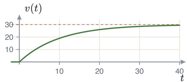
FIGURE 3.28 Example 3.9: v(t) = 30(1 - e^{-t/10}) m/s settles at 30 m/s.
