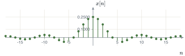
FIGURE 6.19 Its inverse transform, with x[0] = W/\pi = 0.25 .
