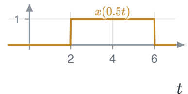
FIGURE 1.15 Stretched: support [2, 6] .
