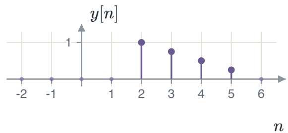
FIGURE 1.11 y[n] = x[n - 2] : every stem moves two samples right. The sample x[1] = 0.75 appears at n = 3 .
