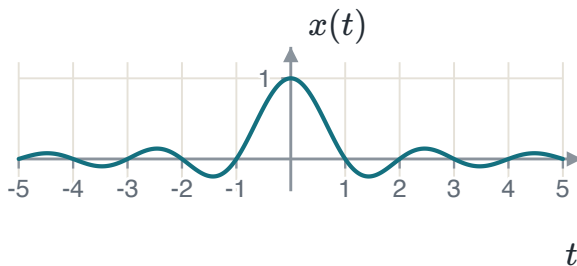
FIGURE 1.64 x(t) = \text{sinc}(\pi t) , with the unnormalised \text{sinc}(\theta) = \sin \theta / \theta . Peak 1 at t = 0 ; zeros at t = \pm 1, \pm 2, \dots
