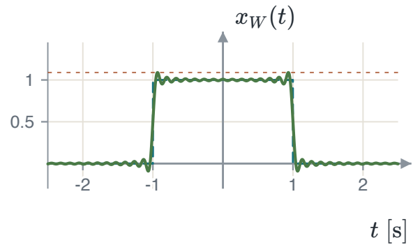
FIGURE 5.6 W = 48 rad/s. The ripples crowd to the jumps; the highest value is 1.089.
