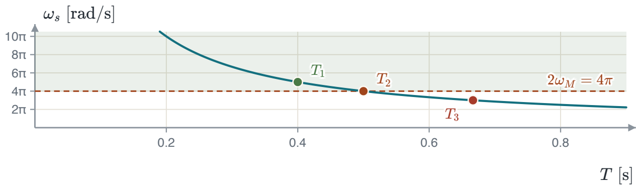
FIGURE 7.13 The rate \omega_s = 2\pi/T against the period T . A period is safe while its point lies above the coral line 2\omega_M = 4\pi rad/s, in the green band.
