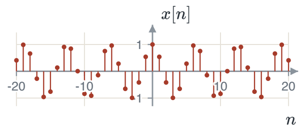
FIGURE 1.50 \cos(n) has \omega_0 = 1 , so \omega_0/2\pi = 1/(2\pi) is irrational. The samples never repeat exactly. It looks periodic, but it is not.
