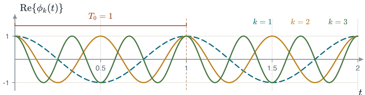
FIGURE 1.52 The harmonics k = 1 (dashed), k = 2 and k = 3 with T_0 = 1 . The k -th makes k full cycles in T_0 , so all of them start together again at t = T_0 .
