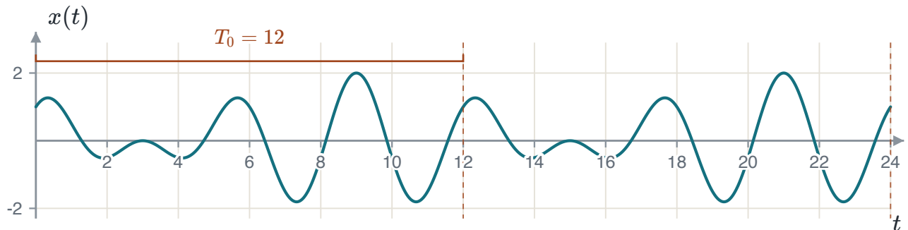
FIGURE 1.22 x(t) = \cos(\frac{2\pi t}{3}) + \sin(\frac{\pi t}{2}) repeats every 12.
