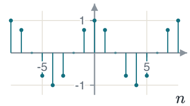
FIGURE 1.48 \omega_0 = 7\pi/4 = 2\pi - \pi/4 : the same samples as \pi/4 .
