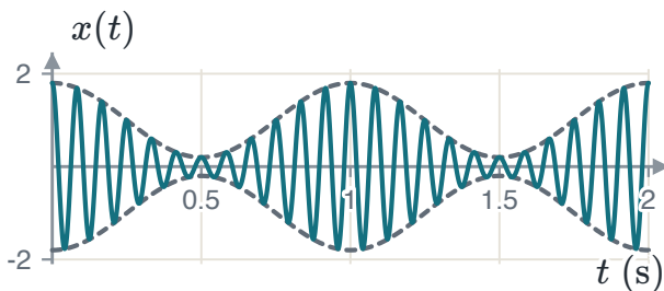
FIGURE 1.71 AM: x(t) = (1 + m \cos(2\pi f_m t)) \cos(2\pi f_c t) with 0 < m \leq 1 . The dashed envelope is \pm(1 + m \cos(2\pi f_m t)) . Drawn with f_c = 12 Hz, f_m = 1 Hz, m = 0.8 .
