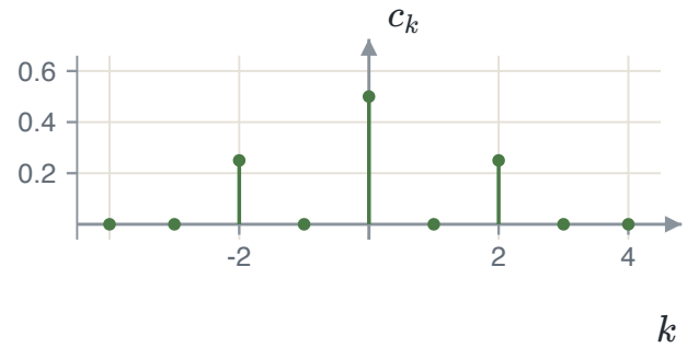
FIGURE 4.56 \cos^2(\omega_0 t) : the pair convolved with itself.
