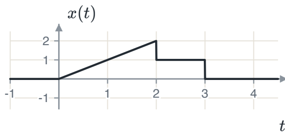
FIGURE 1.35 x(t) : a ramp to 2, a drop to 1 at t = 2 , and a drop to 0 at t = 3 .
