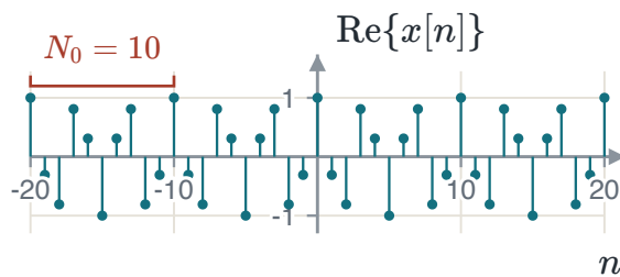
FIGURE 1.49 \text{Re}\{e^{j3\pi n/5}\} repeats every 10 samples.
