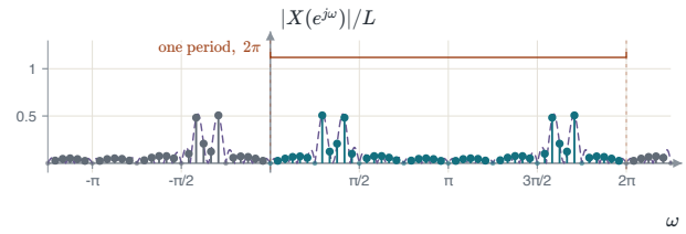
FIGURE 6.12 L = 40 , padded to N = 48 : two separate peaks, at 0.3\pi and 0.4\pi .
