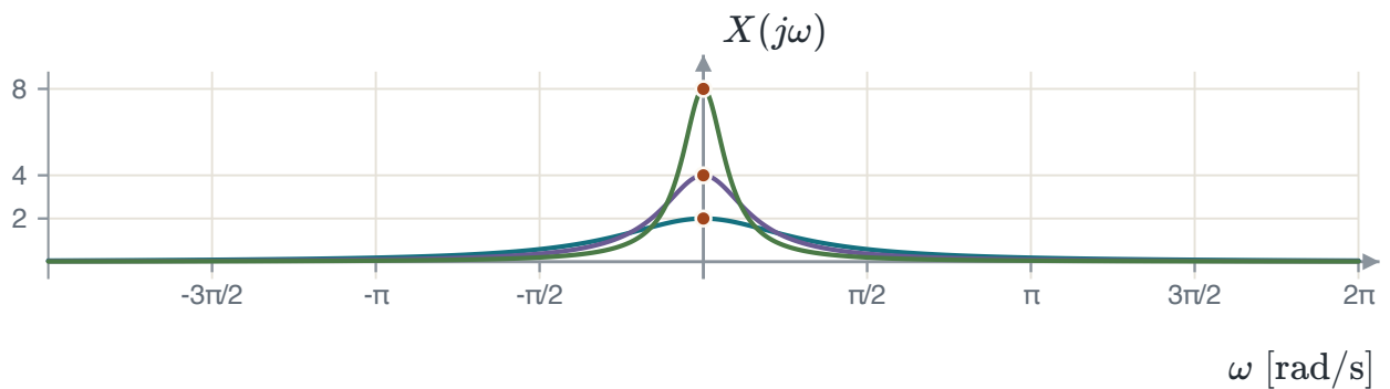
FIGURE 5.7 The transform 2a/(a^2 + \omega^2) for a = 1, 0.5 and 0.25 , with peaks 2, 4 and 8. Every curve has area 2\pi .
