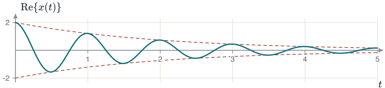
FIGURE 1.41 A damped sinusoid, \text{Re}\{2e^{-0.5t}e^{j2\pi t}\} , with A = 2 , r = -0.5 and \omega_0 = 2\pi rad/s. The envelope \pm 2e^{-0.5t} is dashed.
