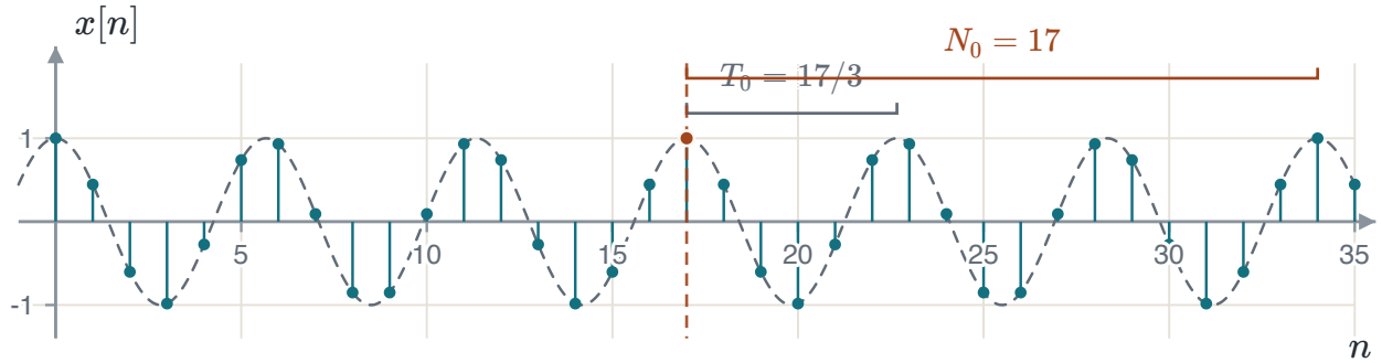
FIGURE 1.51 The dashed curve \cos(6\pi t/17) repeats every 17/3 , but no sample falls at the end of its first or second cycle. After three cycles, at n = 17 , a sample falls on the start of a cycle again. The brackets mark one cycle of the curve and one period of the sequence, both from n = 17 .
