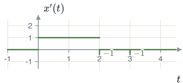
FIGURE 1.36 x'(t) : slope 1 on (0, 2) and two impulses of weight -1 , drawn pointing down.
