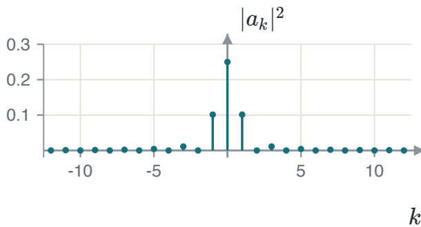
FIGURE 4.62 Power per harmonic of the rectangular wave with T_0 = 4T_1 . The stems add to 0.5.
