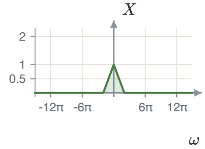
FIGURE 5.26 The filter output: X(j\omega) .
