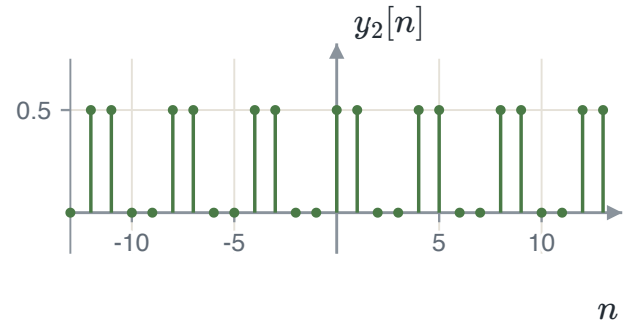
FIGURE 4.75 Low-pass h_2 : the average remains.
