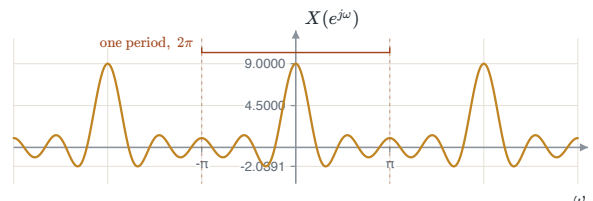
N_1 = 4 : peak 9, least value -2.0391 , and a main lobe half as wide.
