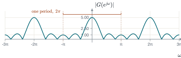
|G(e^{j\omega})| : peak 5, and the finite value 1 at \omega = \pi .
