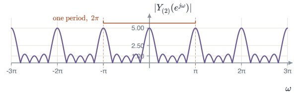
|Y_{(2)}(e^{j\omega})| : the same picture twice inside every 2\pi .
