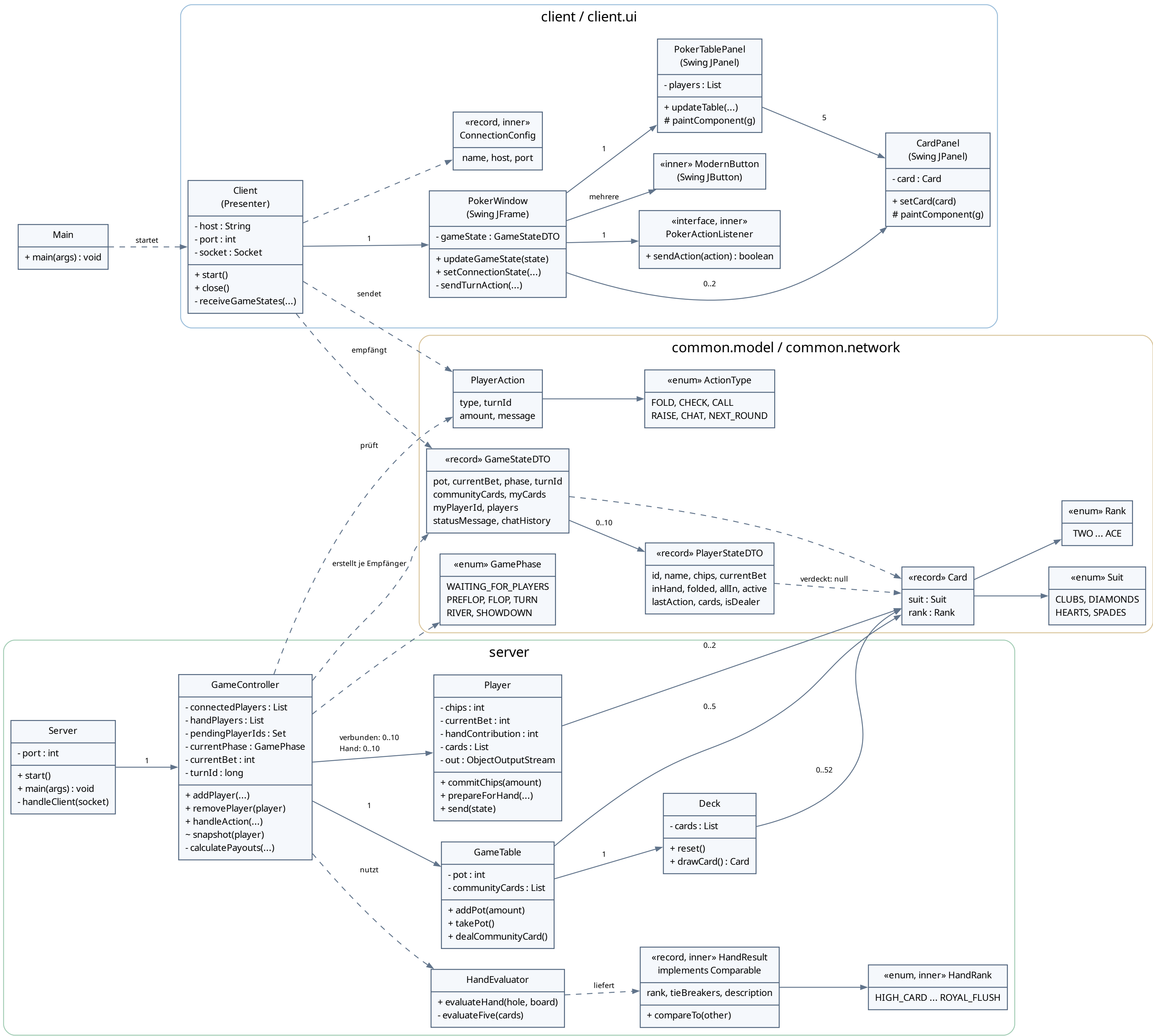
OpenPoker — Klassendiagramm
