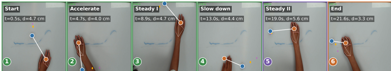
(a) Key deployment frames matched to panel (b) video frames from first rollout; numbered times match the ZPD plot
