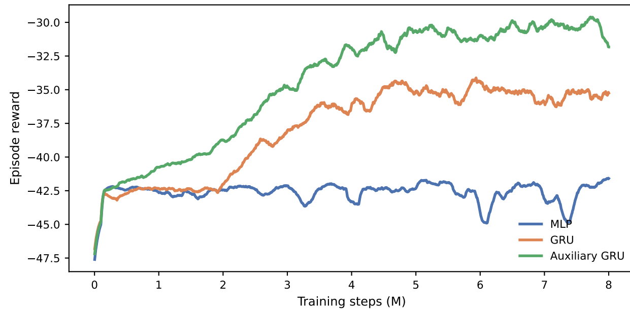
(a) Reward during GRU ablation
