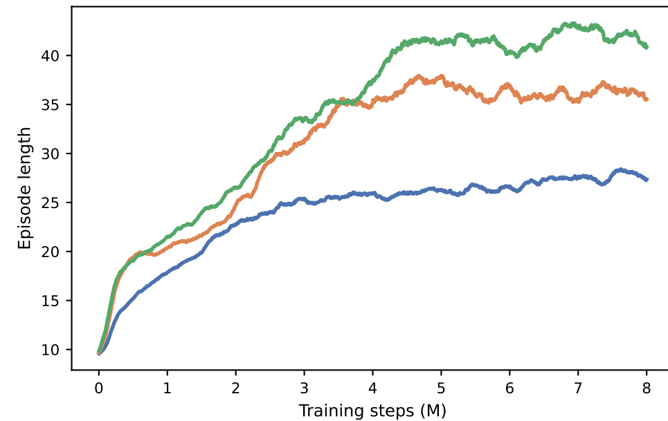
(b) Episode length during GRU ablation
