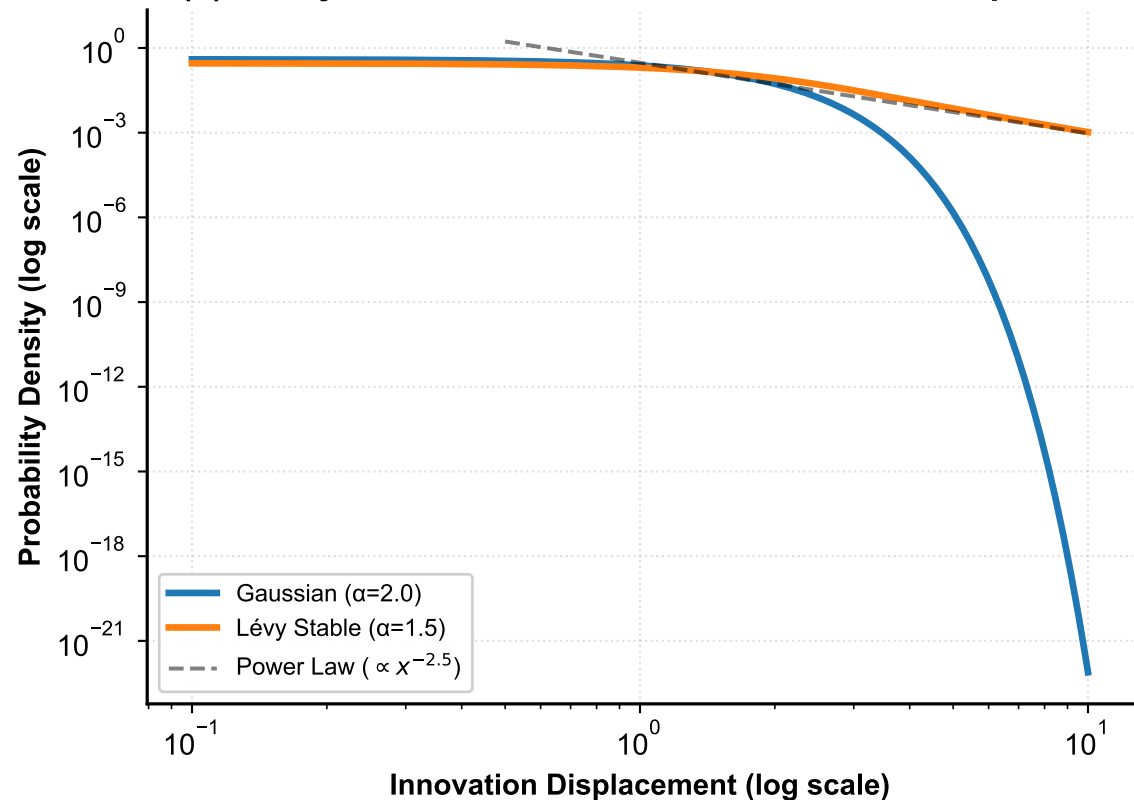
(b) Heavy-Tailed Behaviour of the Innovation Sequence
