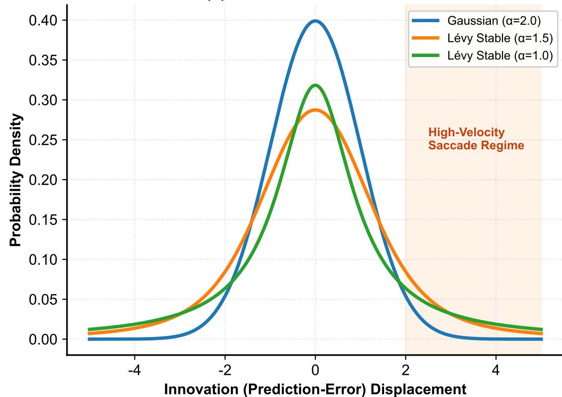
(a) Innovation Distribution
