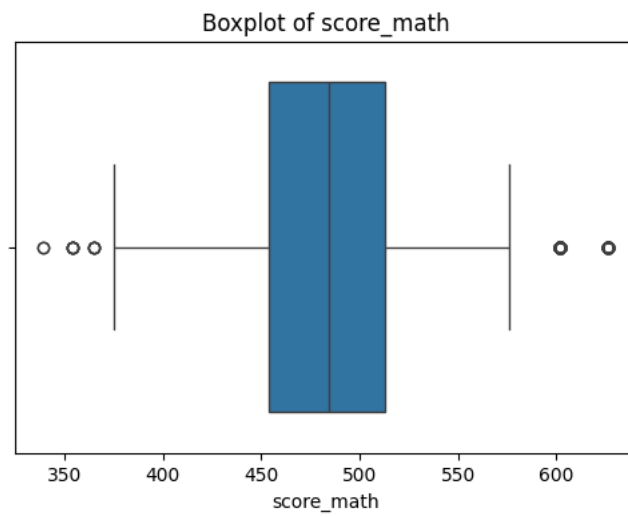
Figure 20: Boxplot of Outliers for score_math
