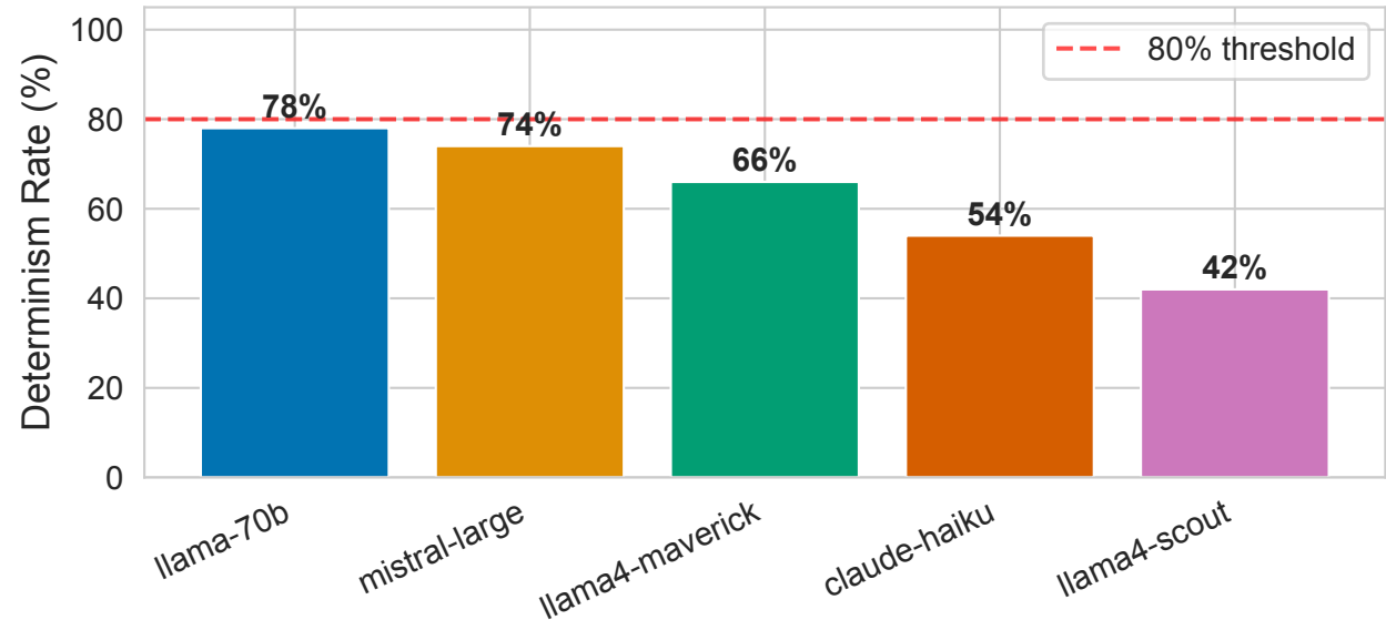
Model Determinism at Temperature 0 (50 MMLU Questions × 30 Reps)
