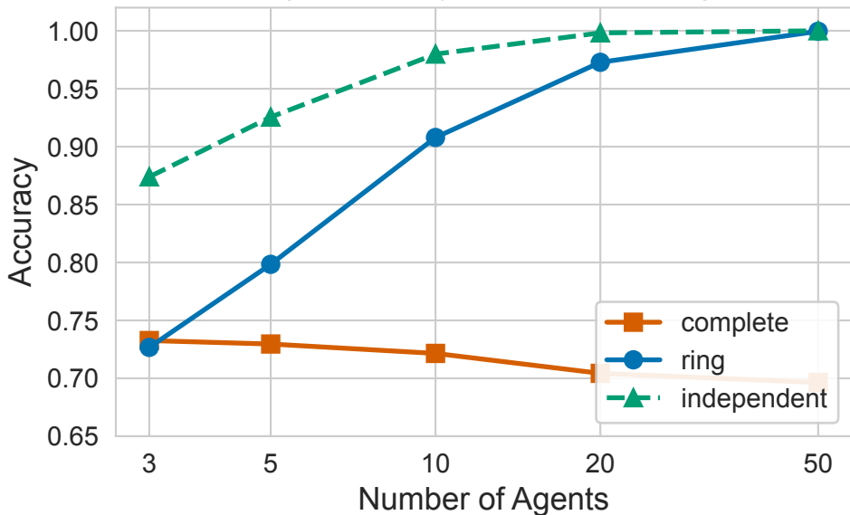
Scaling: Accuracy vs Number of Agents
