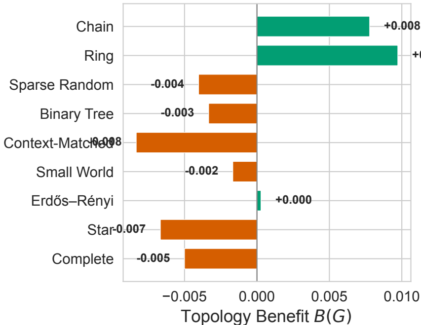
(a) Benefit vs Independent Baseline
