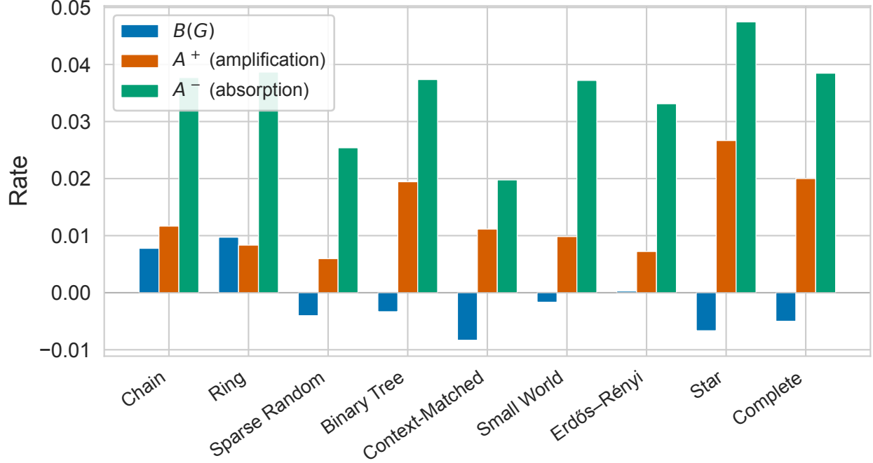
Amplification–Absorption Decomposition (Phase 2a: 5 LLMs × 100 MMLU Questions)
