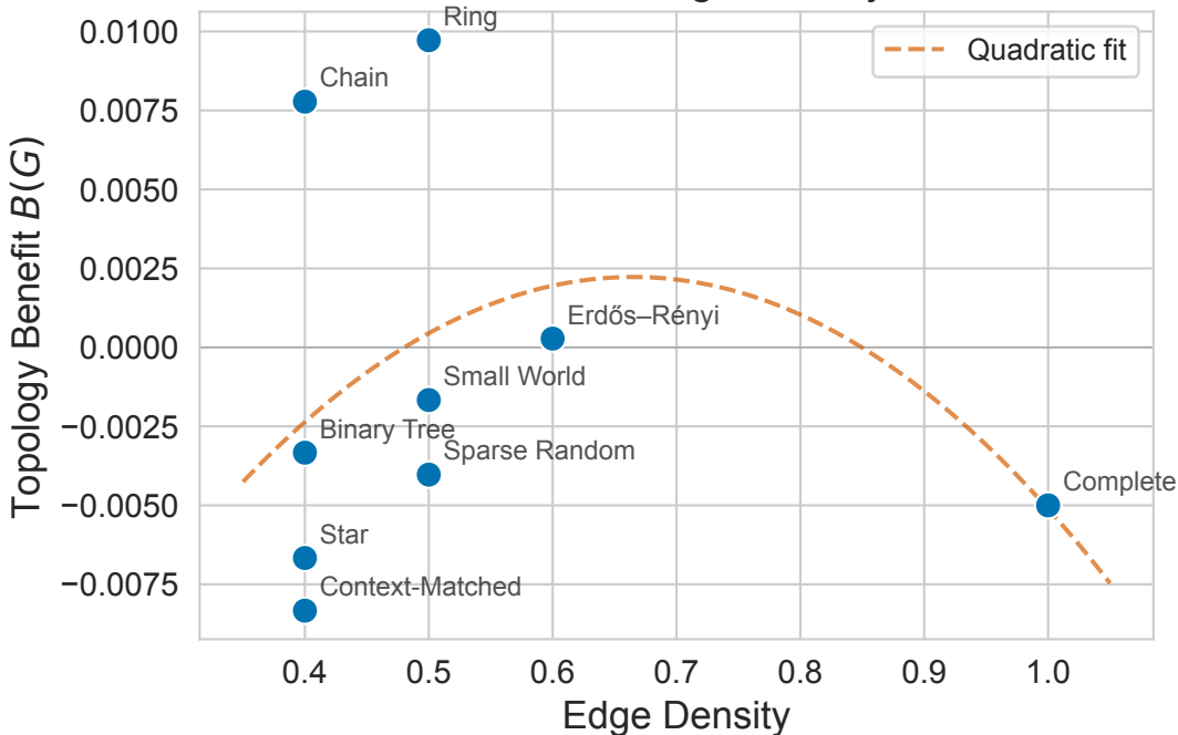
Phase Transition: Edge Density vs B(G)
