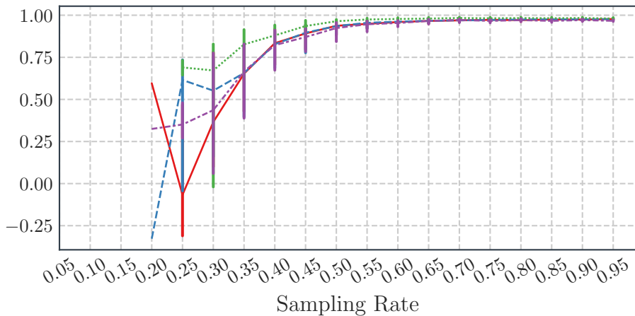
P50 of R2 Scores +/- to P80 and P20
