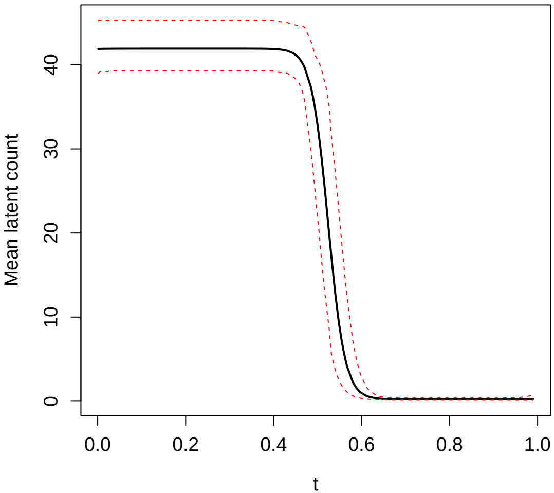
data 2: gene 1
