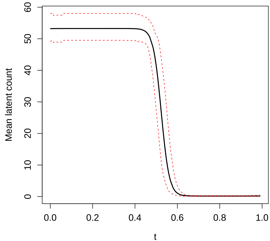
data 2: gene 2
