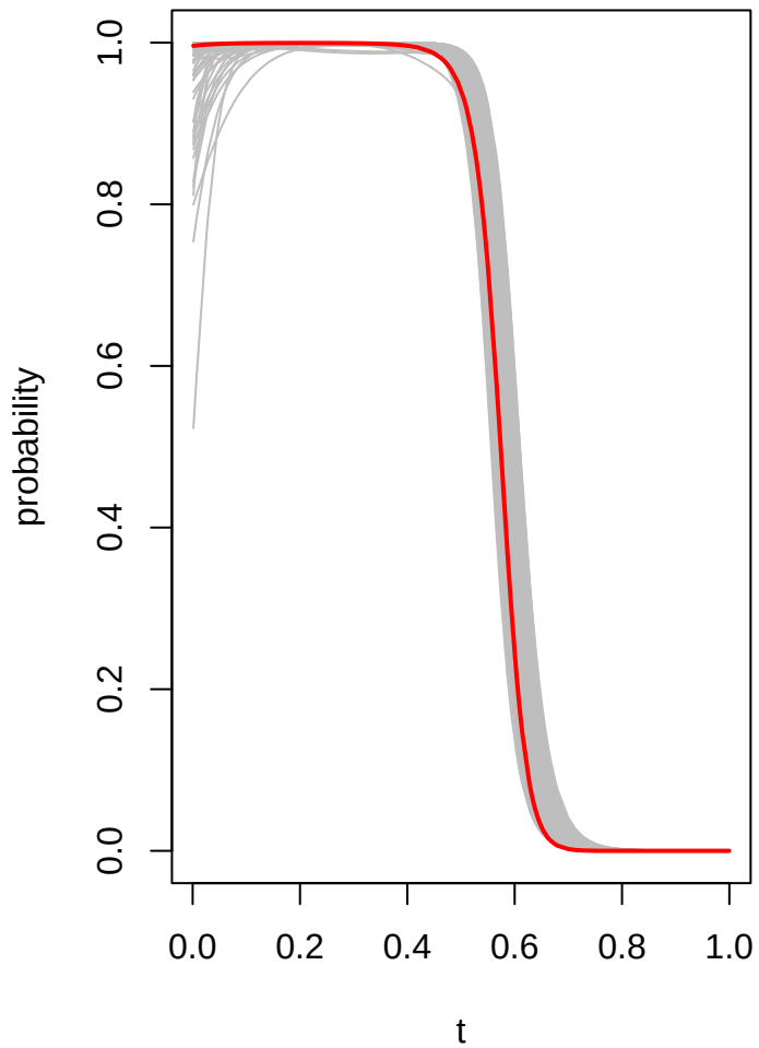
data 1: cluster 2
