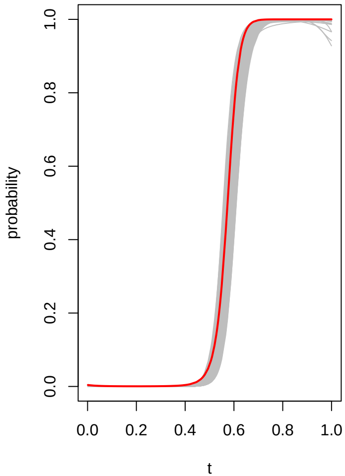
data 1: cluster 1
