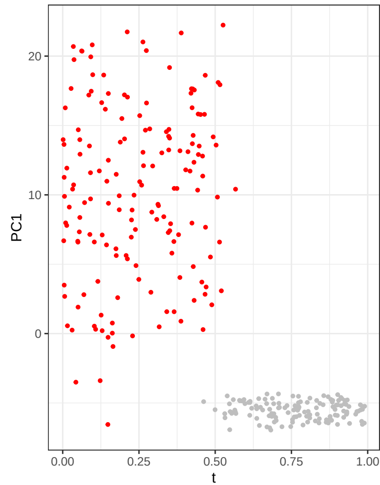
data 2: Cluster 3
