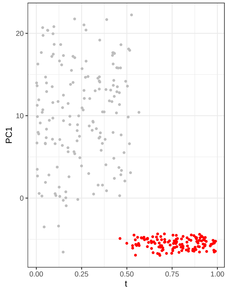
data 2: Cluster 2
