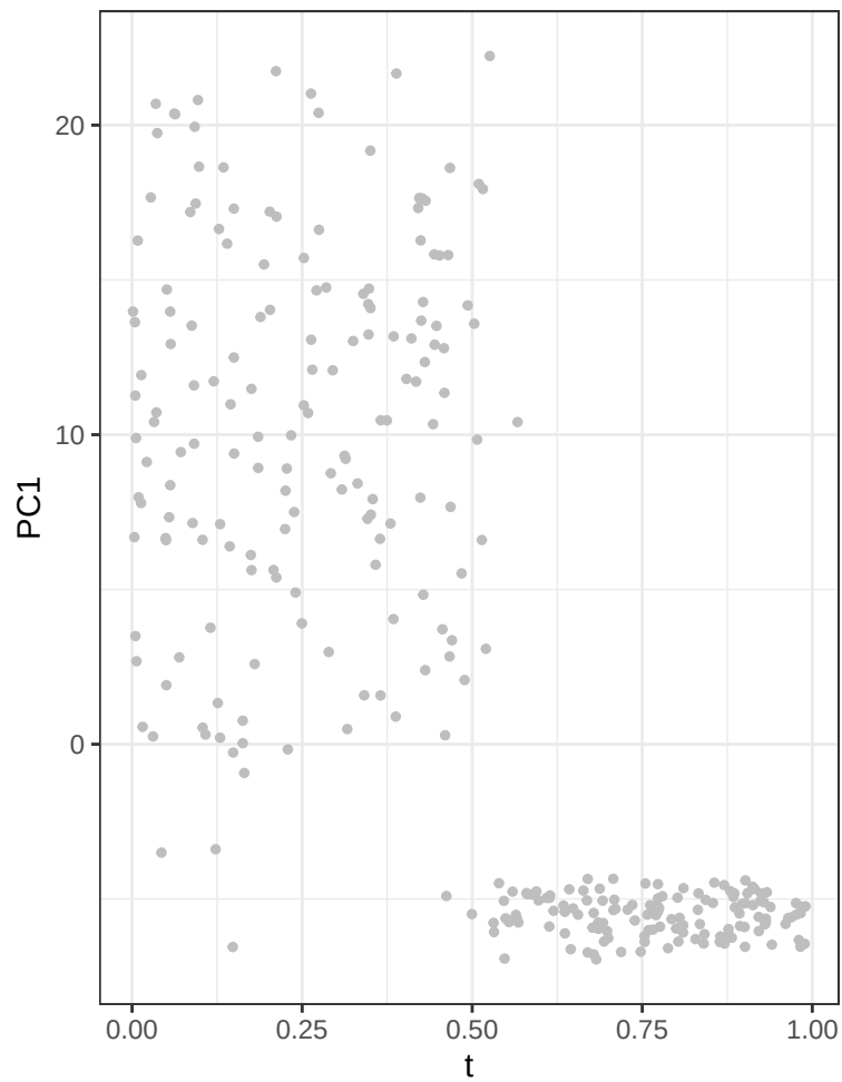
data 2: Cluster 1
