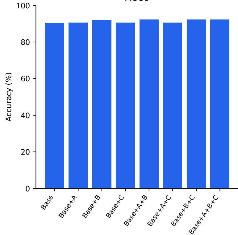
ACC8
