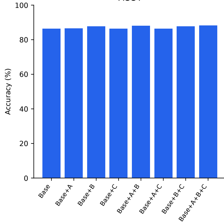
ACC4
