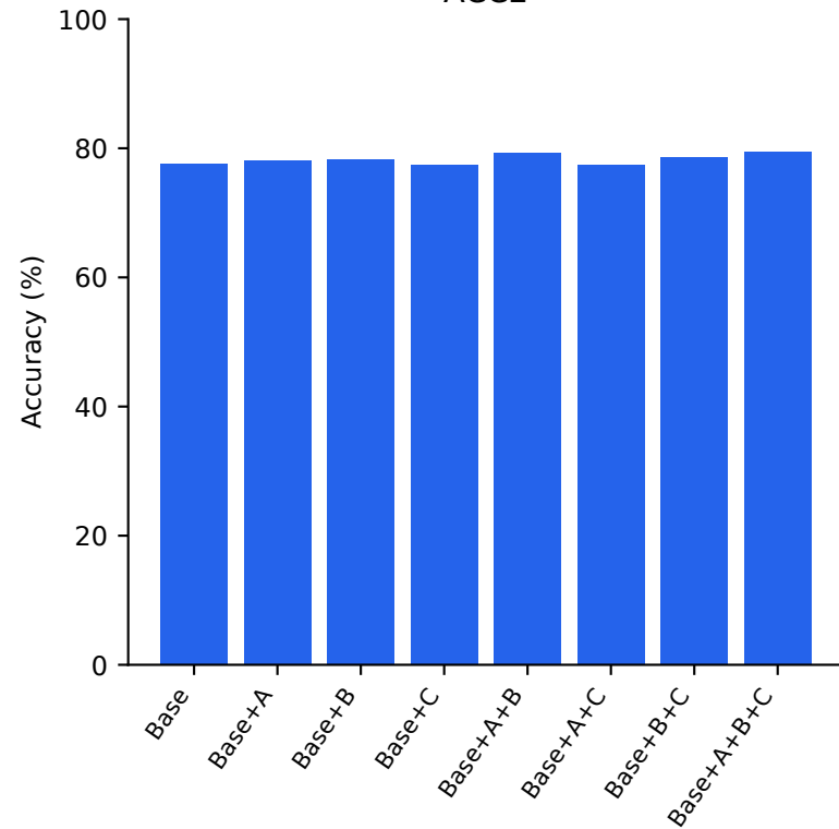
ACC2
