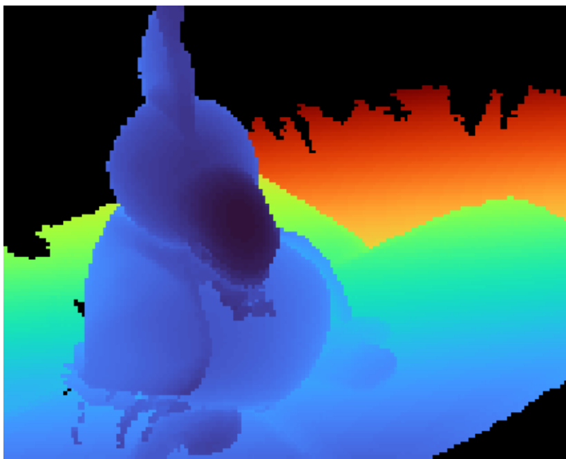
Base+A+B+C depth
