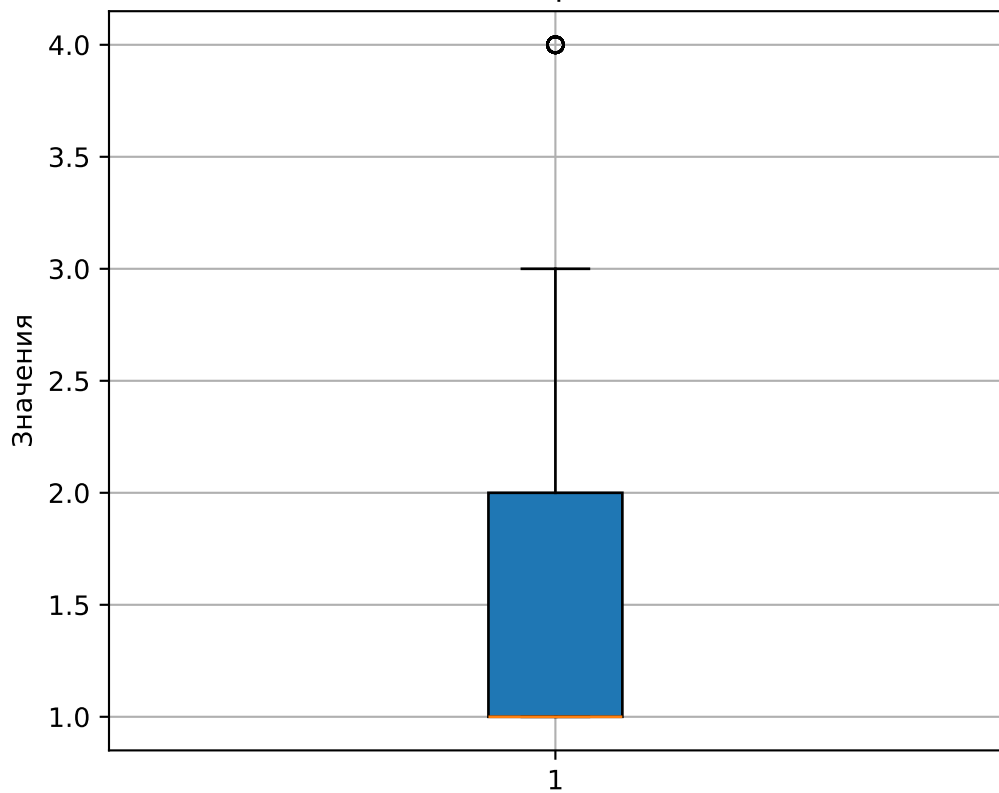
Boxplot
