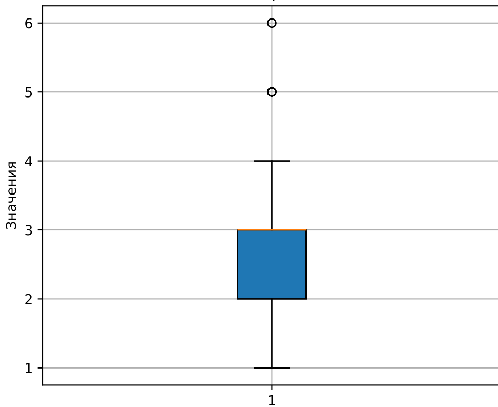
Boxplot
