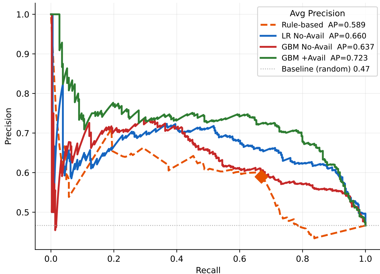
Precision-Recall Curve (OOF)
