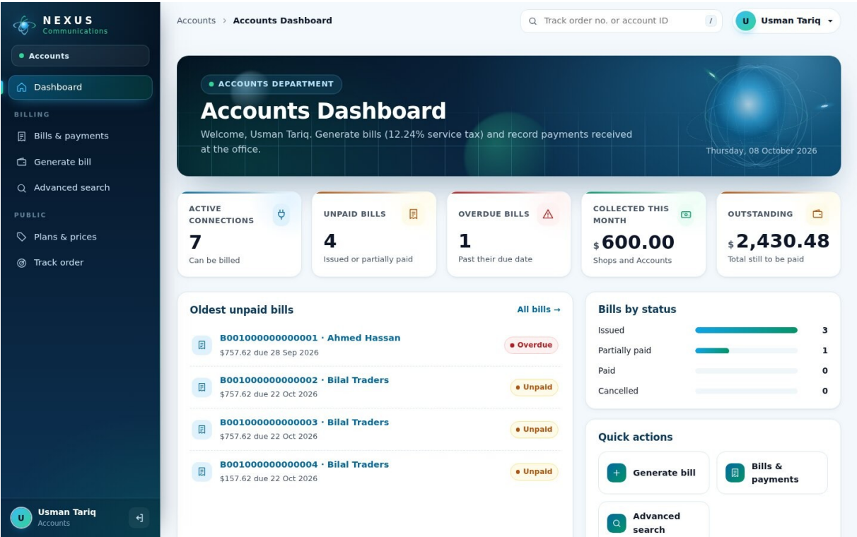
Figure 33. Accounts dashboard
