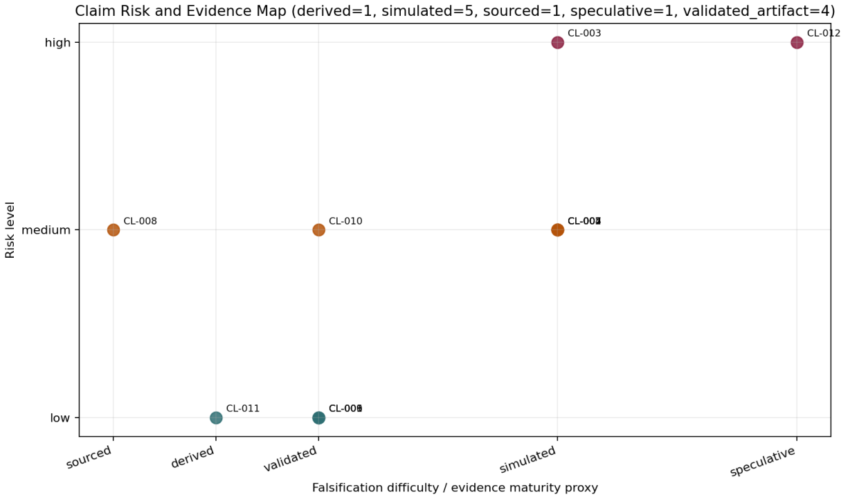
Figure 6: Robust, sensitive, and speculative claims mapped against falsification difficulty.
