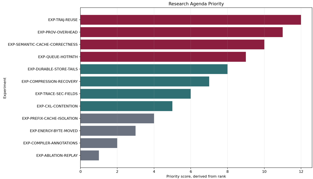
Figure 5: Ranked prototype/research experiments by priority and uncertainty reduction.
