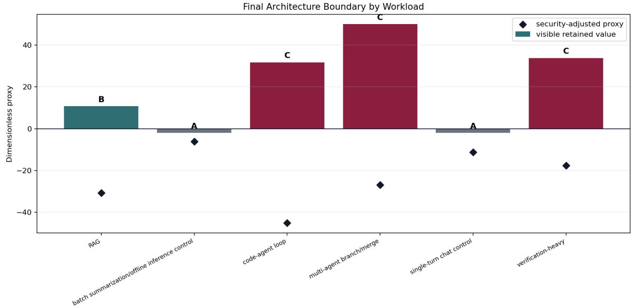
Figure 4: Final Option A/B/C decision by workload after queueing, compression, calibration, and security gates.
