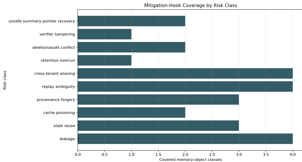
Figure 2: Mitigation-hook coverage for each security/provenance risk class.
