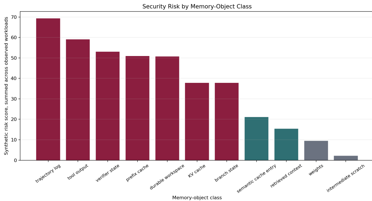
Figure 1: Synthetic security risk score by memory-object class, summed across observed workloads.
