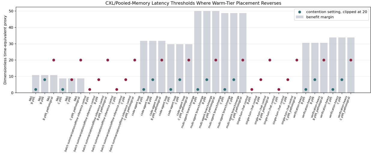
Figure 2: CXL/pooled-memory latency thresholds where warm-tier placement reverses.
