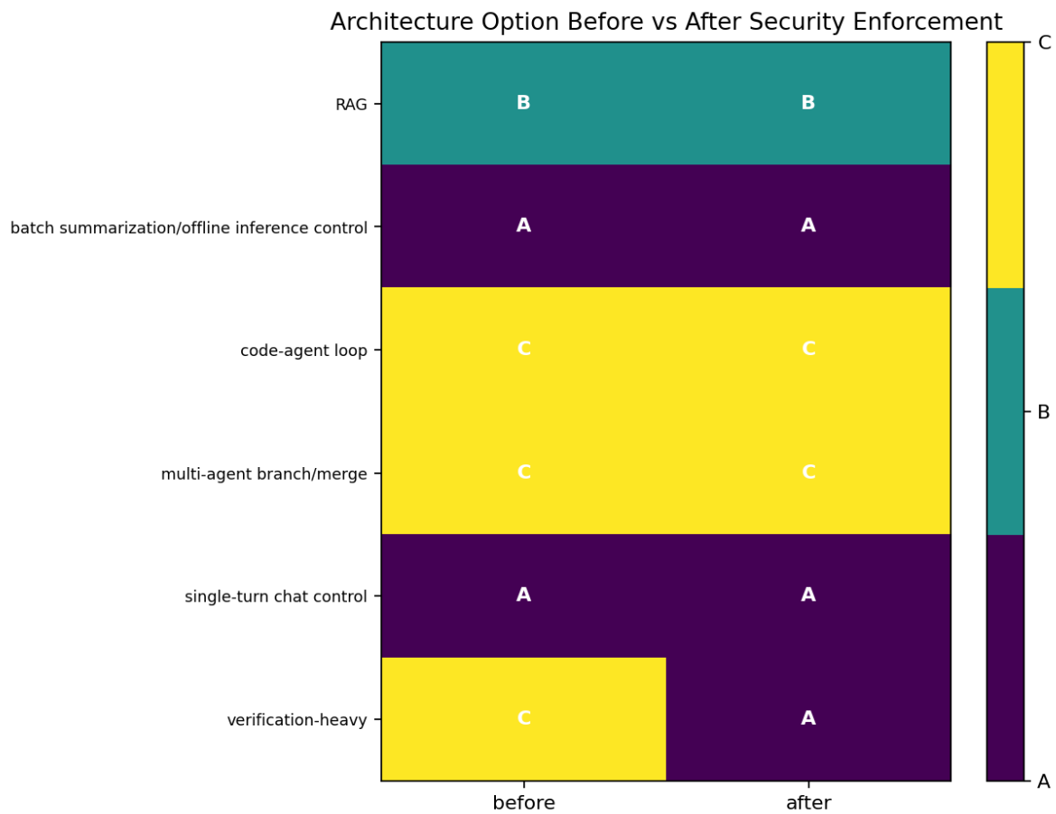
Figure 6: Architecture options before and after enforcement show controls staying Option A and verification-heavy collapsing from Option C to Option A under synthetic enforcement loss.
