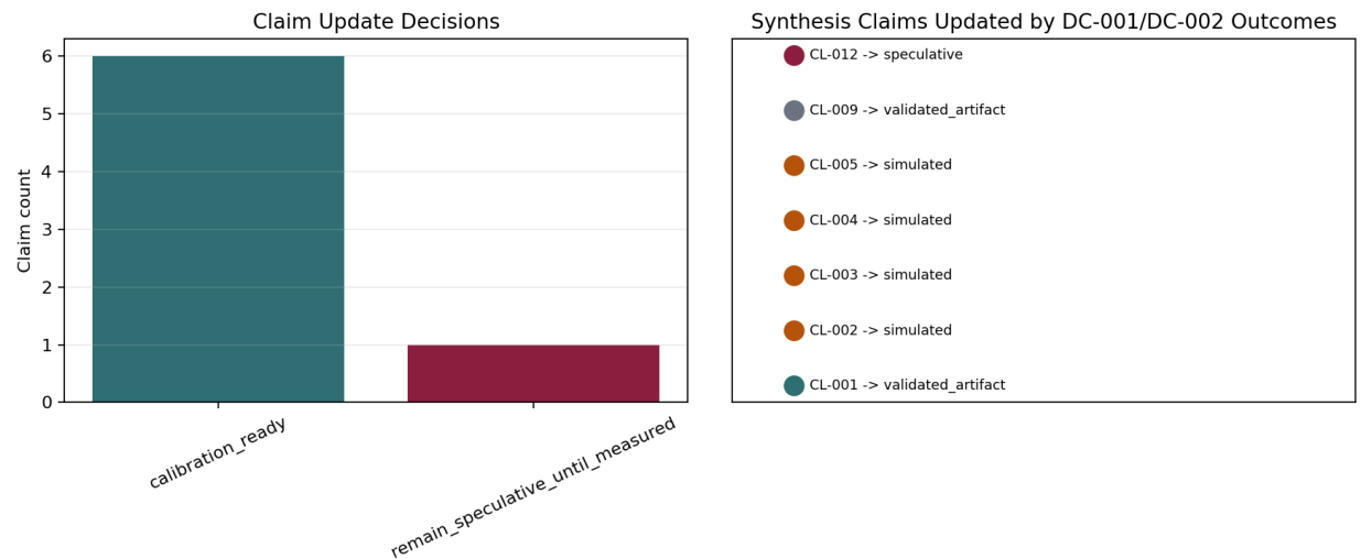
Figure 3: Synthesis claims updated by DC-001/DC-002 measurement outcomes.
