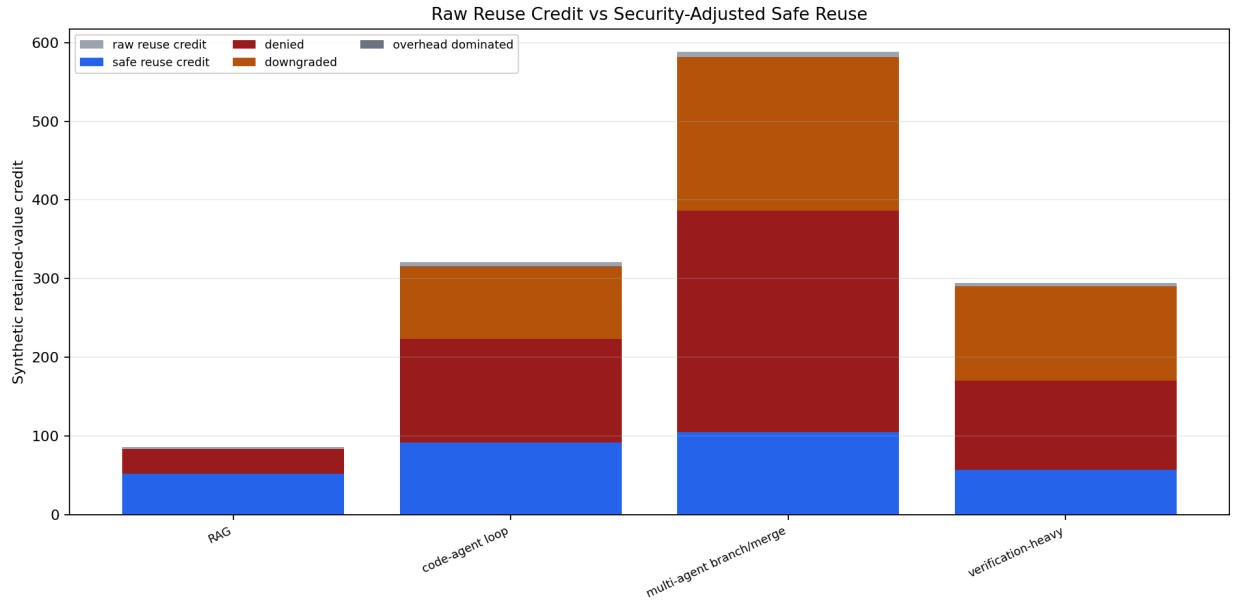
Figure 4: Raw reuse credit is split into safe, denied, downgraded, and overhead-dominated retained-value credit by workload.
