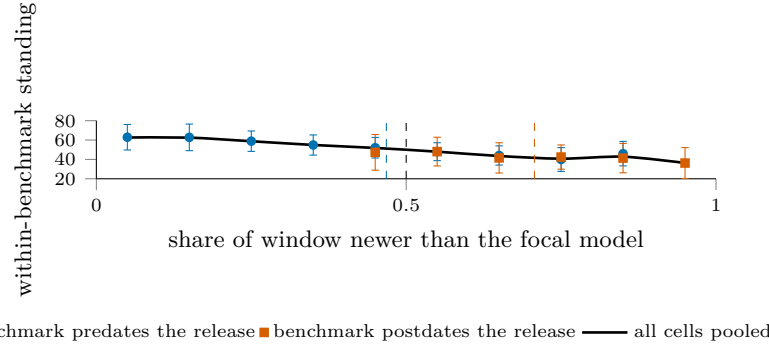
Figure 2: Standing against the share of a cell’s window released after the focal model; dashed verticals mark group mean shares, the black dashed line the symmetric 0.5. Eligible and placebo cells lie on one declining curve, so the contrast between them is a position on the curve, not a fact about disclosure. Intervals clustered on organisation.
