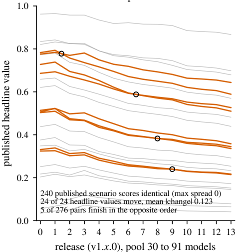
HELM Lite: headline is Mean win rate, which is pool-relative
