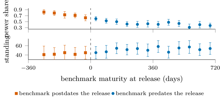
Figure 1: The mechanism and the outcome at the availability boundary. Top: the share of a cell’s comparison window released after the focal model, against benchmark maturity at release; it falls with maturity and jumps at the boundary. Bottom: within-benchmark standing on the same axis, continuous through it. Sixty-day bins; intervals clustered on organisation.
