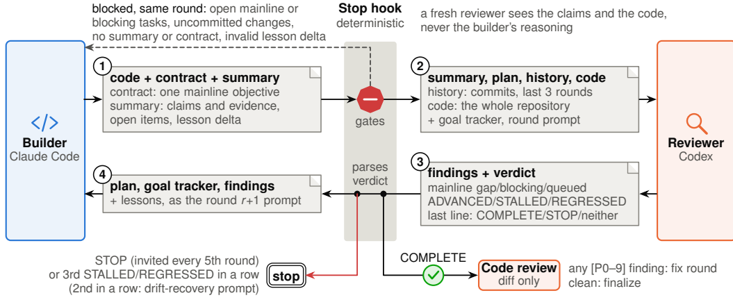
Figure 4: Humanize’s Stop hook makes each RLCR round an evidence-based builder–reviewer exchange. (1) The builder submits code, a round contract, and a claim summary. (2) After the hook’s gates pass, a fresh reviewer checks the claims against the plan, history, and code. (3) The reviewer returns findings and a verdict. (4) The hook uses them to prompt the next round, start code review, or stop the loop.
