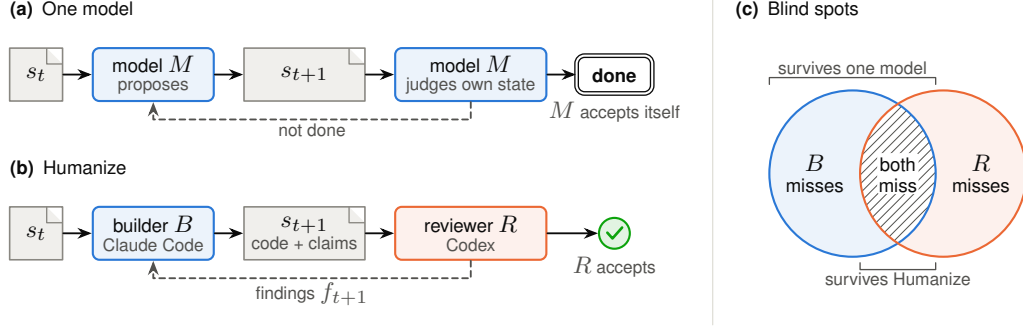
Figure 2: Alternating models reduces accepted defects when their blind spots differ. (a) One model M proposes and judges each state, leaving its blind spots unchecked. (b) Humanize forms a joint sampler: builder B proposes each state, and reviewer R from another vendor judges it and decides acceptance. (c) A defect overlooked by B survives the loop if R also misses it.
