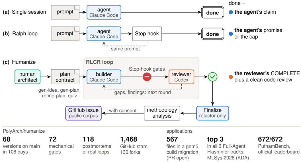
Figure 1: Humanize separates building from acceptance through independent review and mechanical gates. (a)–(c) The right column compares who declares completion in a single session, a Ralph loop (Huntley, 2025), and Humanize. In (c), Stop-hook gates and an independent reviewer check each builder round; dashed arrows return work. The bottom strip summarizes the project’s development record and applications.
