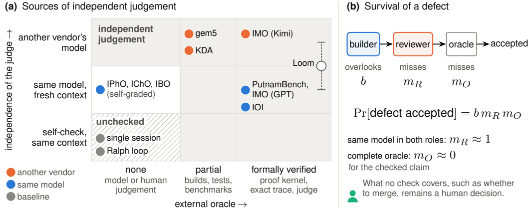
Figure 6: Independent judgement can come from a second model or an external oracle. (a) Applications and baselines are positioned by reviewer independence and oracle strength; acceptance is unchecked when both are absent. (b) A defect is accepted with probability b m_R m_O . A reviewer from another vendor can lower m_R ; a complete oracle drives m_O toward zero for the claim it checks.
