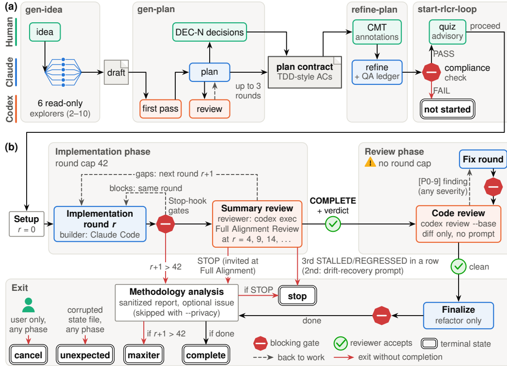
Figure 3: Humanize fixes the plan before execution and makes completion a reviewer decision. (a) The planning chain separates human, Claude, and Codex roles. Lanes denote actors, regions denote commands, and the first three commands are optional. (b) The RLCR state machine shows default transitions and explicit exits. Octagons mark blocking gates; dashed arrows return work; red arrows exit without completion.
