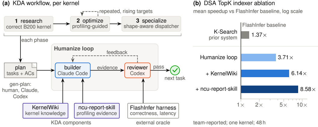
Figure 5: Kernel knowledge and profiling feedback improve KDA’s reported DSA indexer speedup. (a) The builder queries KernelWiki for production kernels, contest submissions, and documentation, and uses ncu-report-skill to interpret Nsight Compute profiles. The reviewer checks this evidence against each acceptance criterion, using the official FlashInfer harness as oracle. (b) The team-reported 48-hour DSA TopK indexer ablation adds each component to the Humanize loop. K-Search is a separate prior system.
